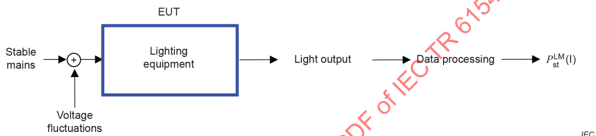
Figure 6 – Measuring P_{st}^{LM(I)}
