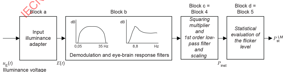
Figure A.2 – Structure of the light flickermeter based on a modified voltage flickermeter
