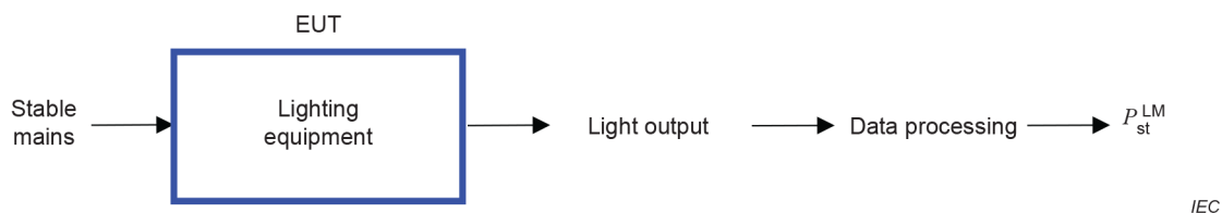
Figure 5 – Measuring P_{st}^{LM}
