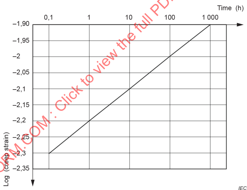
Figure 1 – Typical creep curve
