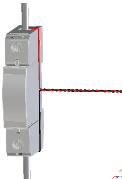
Figure 6 – Routing of the measurement lines of an SPD having a single mode of protection
