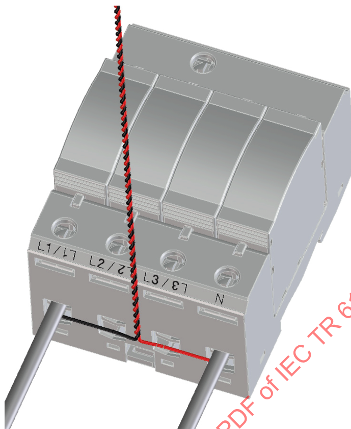
Figure 8 – Routing of the measurement lines of a multimode SPD, example 1
