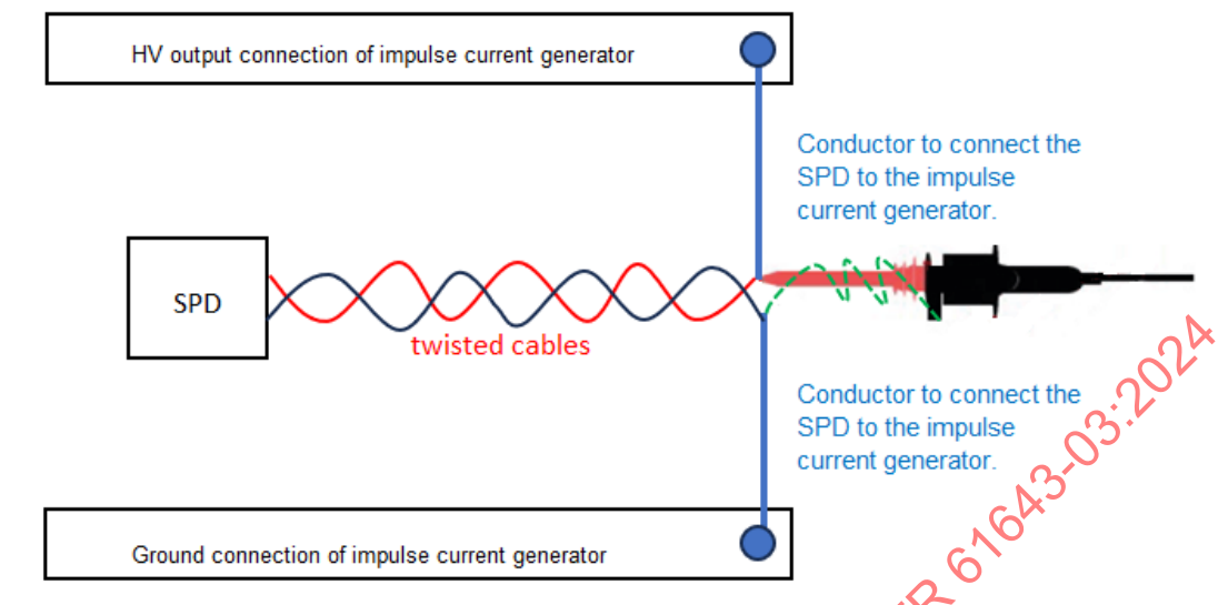
Figure 11 – Example for the application of method 1 and method 2 where the SPD is provided with pigtail connections
