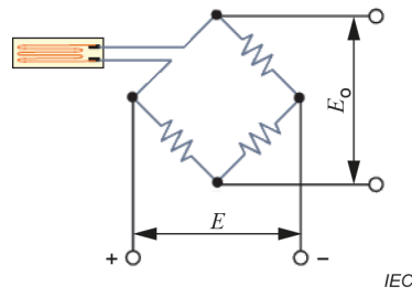
Figure 8 – Resistor bridge for strain measurement
