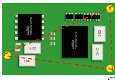
Figure 7 – Strain during screwing
