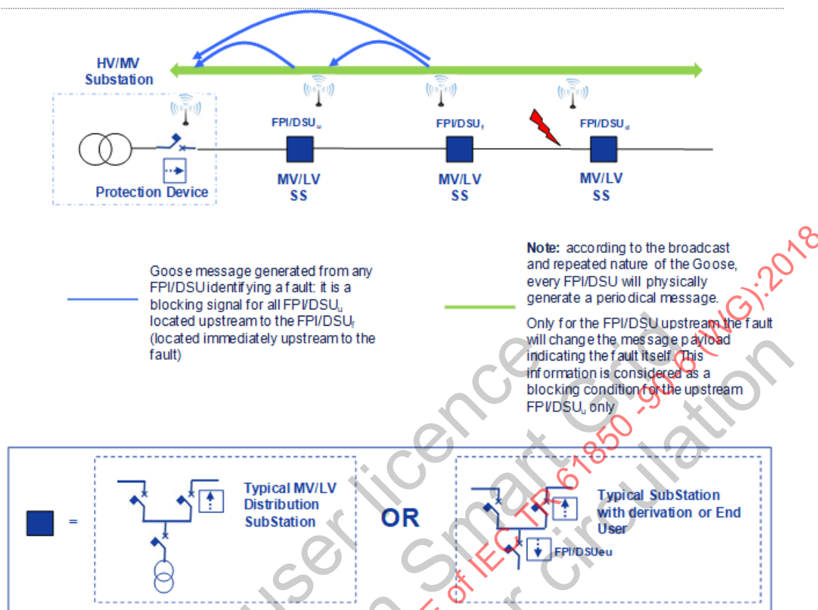
Figure 40 – Logical selectivity – FLI along the MV feeder
