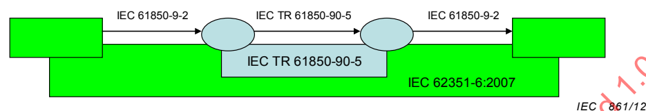
Figure 20 – End-to-end cryptographic integrity for IEC 61850-9-2 implementations
