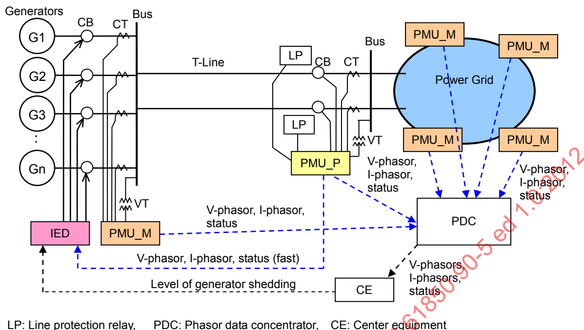
Figure 10 – Use case diagram for WAMPAC
