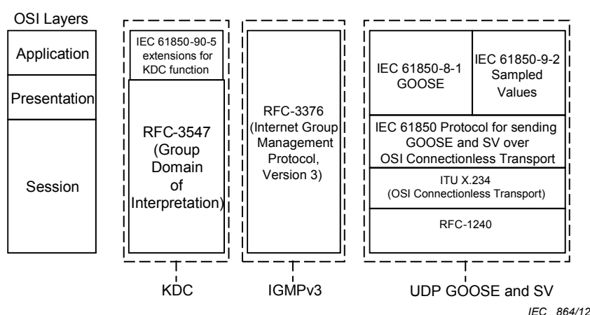
Figure 23 – IEC/TR 61850-90-5 A-Profiles
