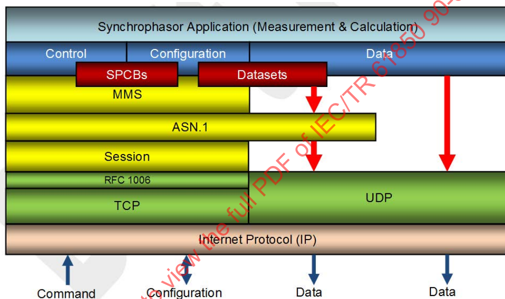
Figure 22 – General service mappings
