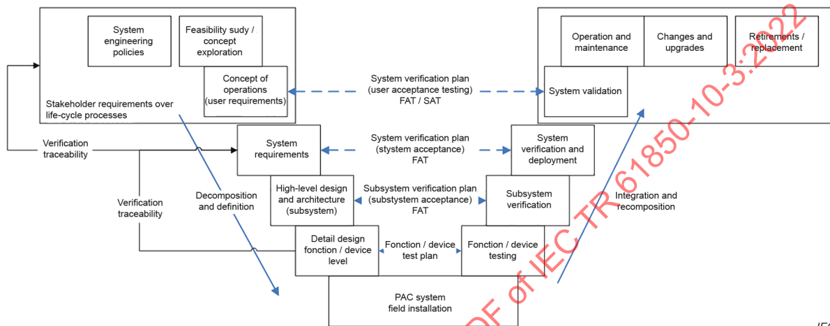
Figure 13 – V-Model used for system engineering
