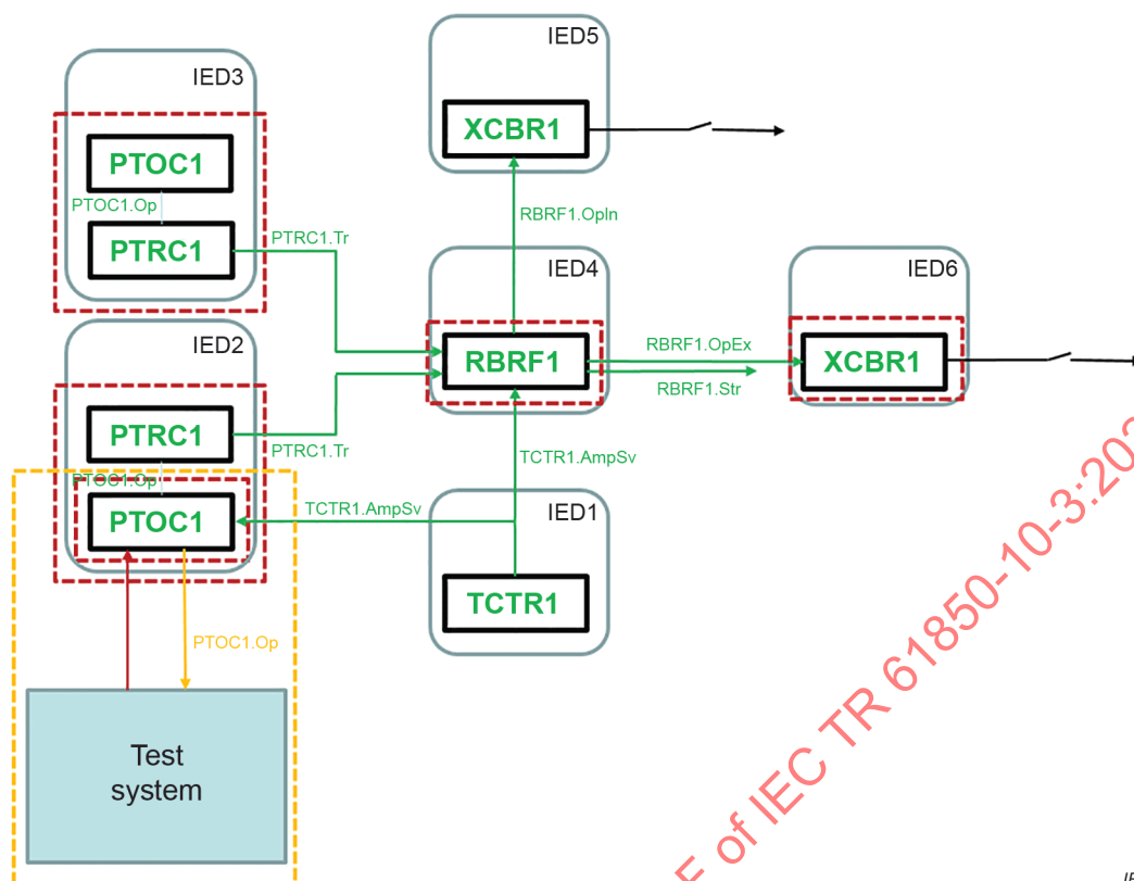
Figure 30 – Interfaces between test system and tested IED for testing of line protection function
