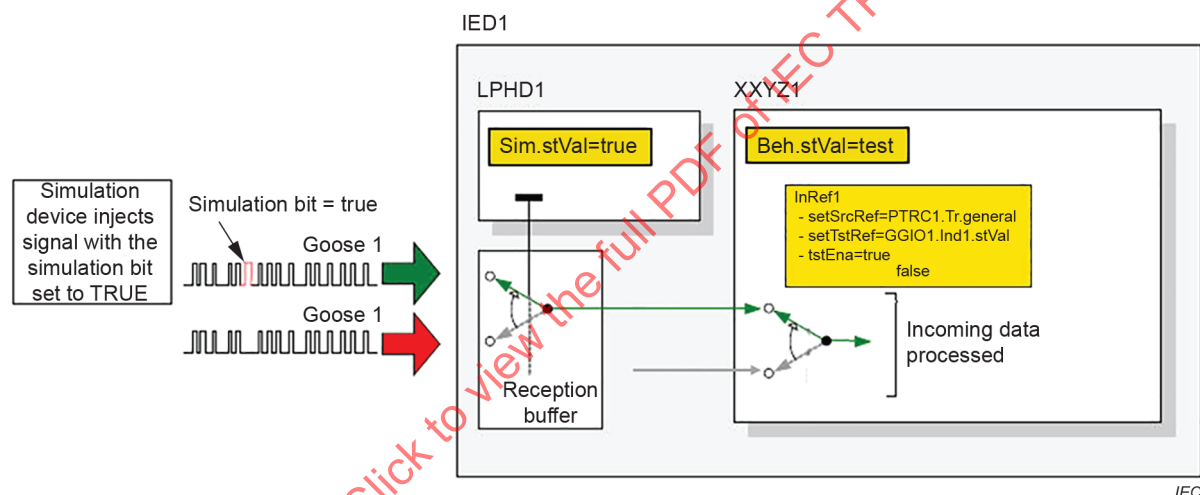
Figure 10 – Use of InRef for LN test
