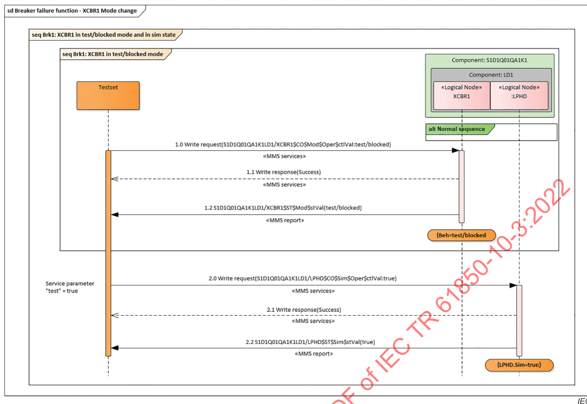
Figure 27 – Breaker function: Setting the mode and the simulation state
