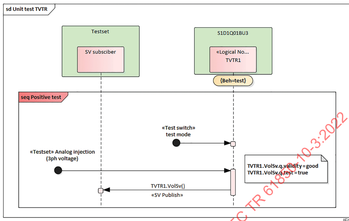
Figure 38 – Unit test of TVTR LN
