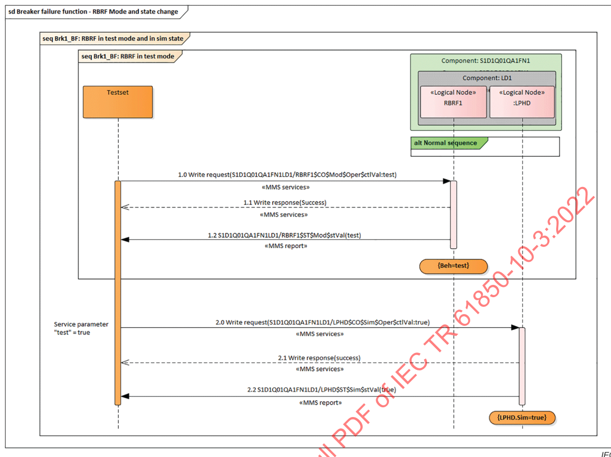
Figure 26 – Breaker failure function: Setting the mode and the simulation state
