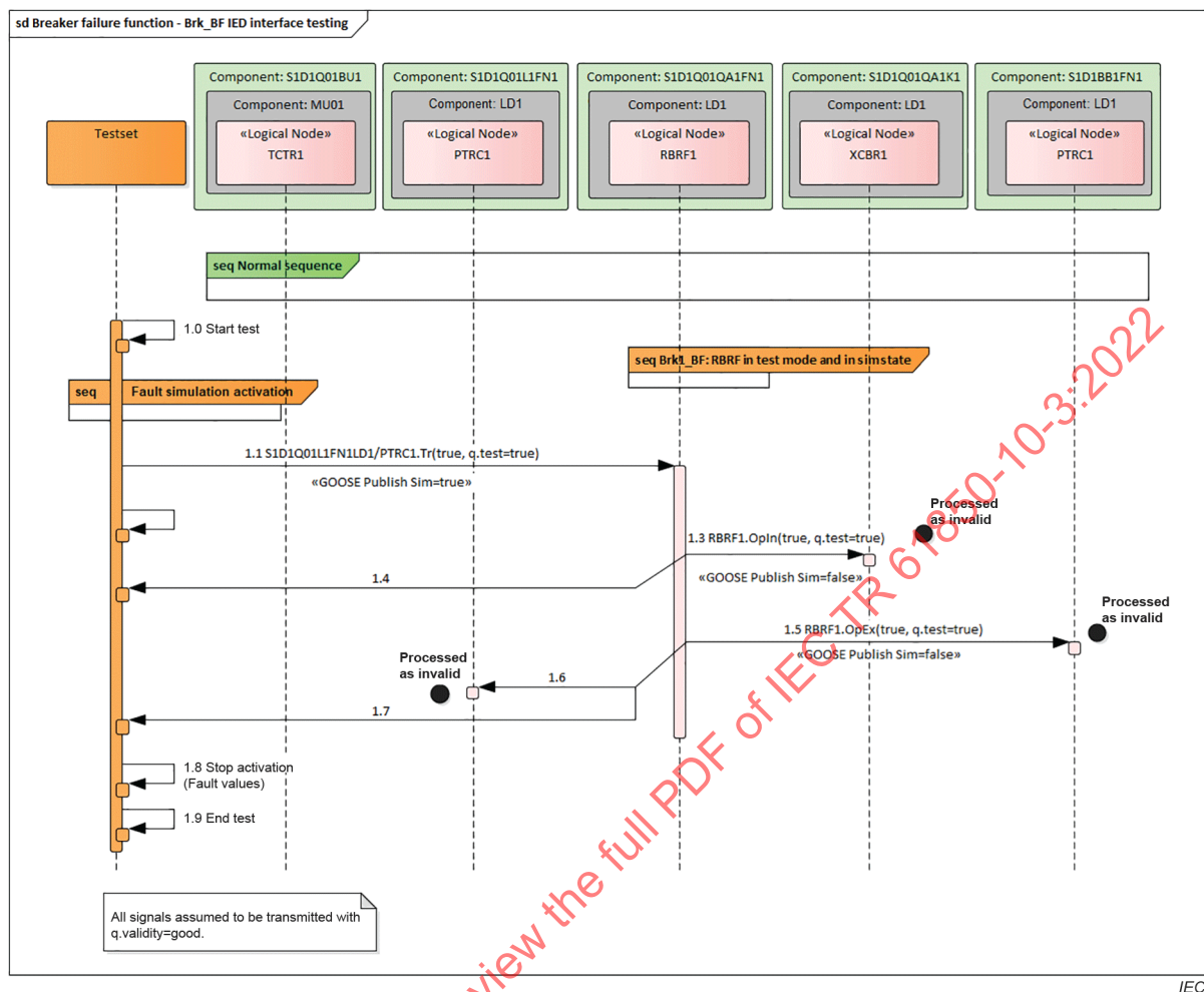
Figure 31 — Breaker failure IED A interface testing
