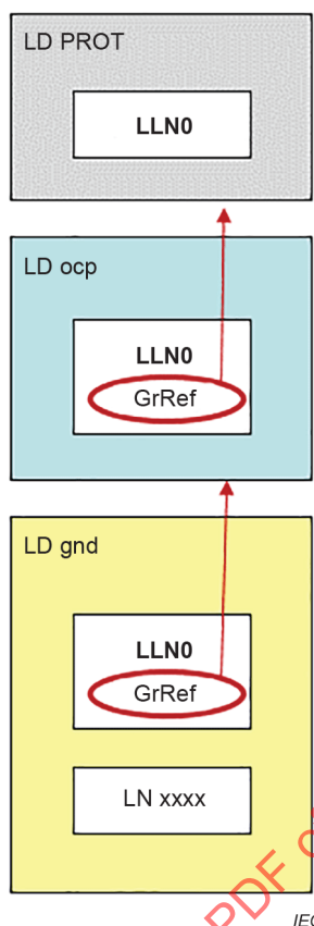
Figure 5 – Use of GrRef in the modelling of nested logical devices
