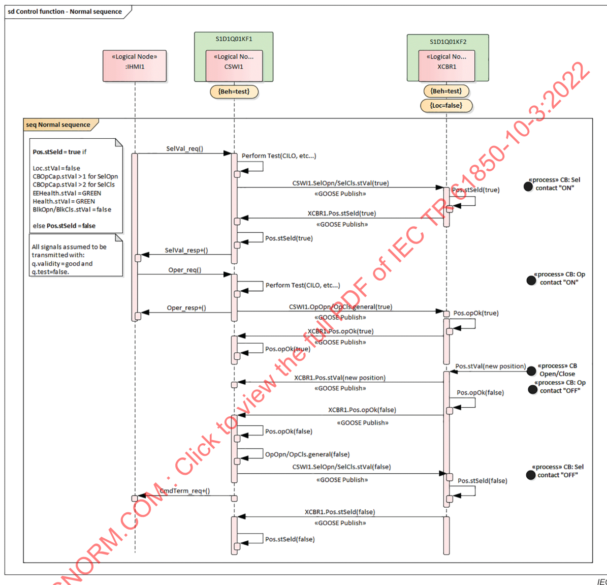
Figure 21 – Simplified SBO scheme behaviour
