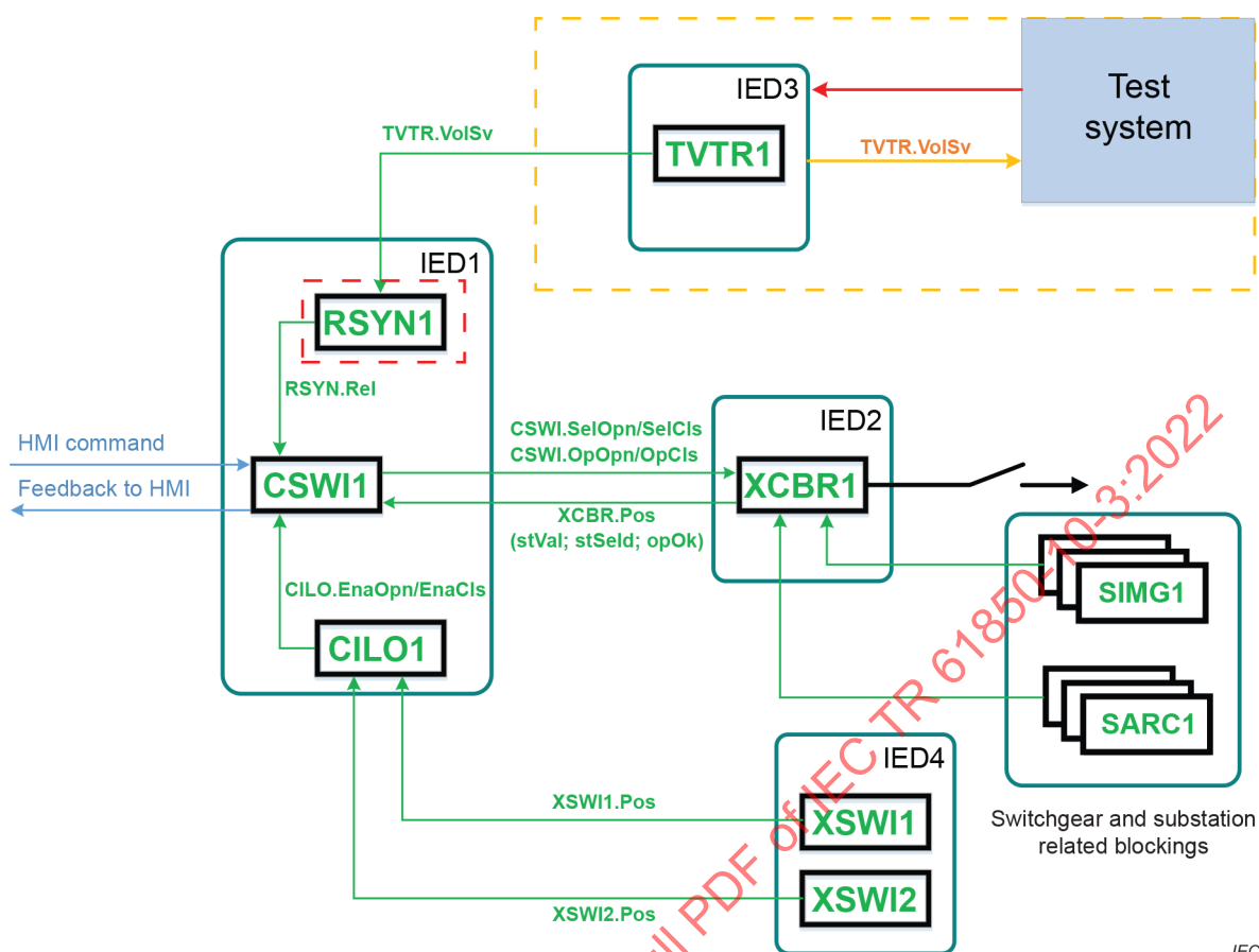
Figure 37 – Unit test of TVTR LN – simplified
