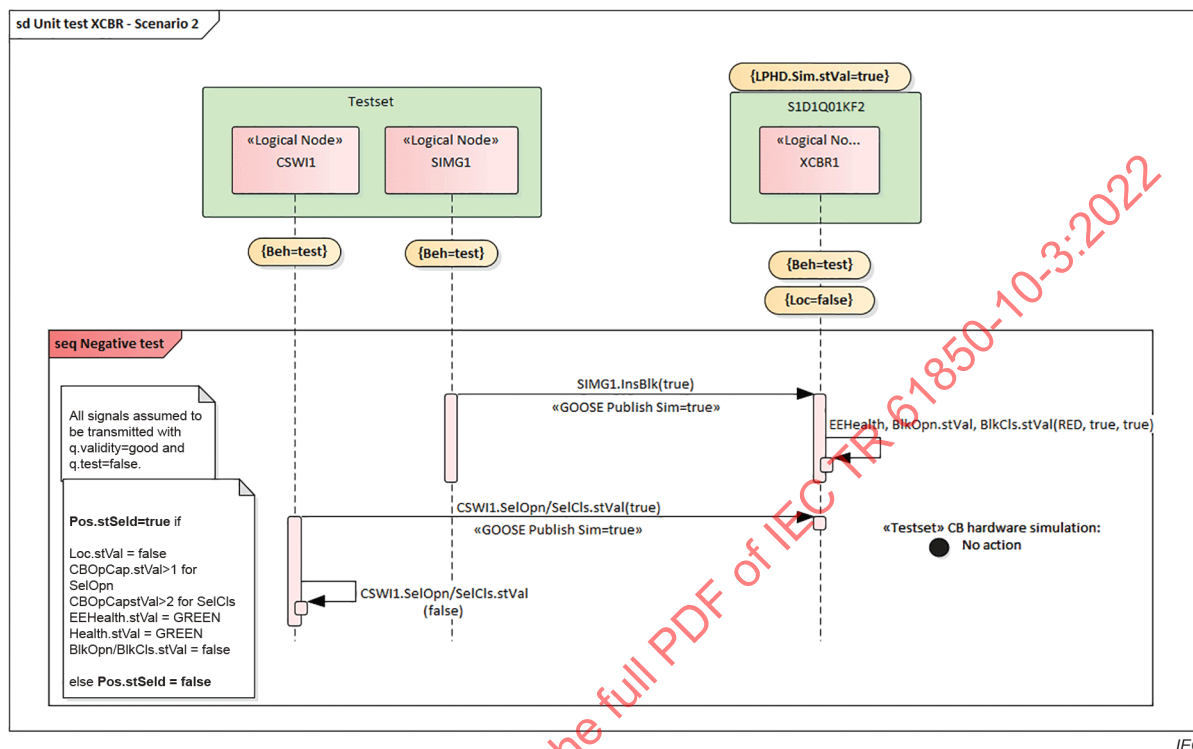
Figure 42 – Unit test of XCBR LN – Scenario 2
