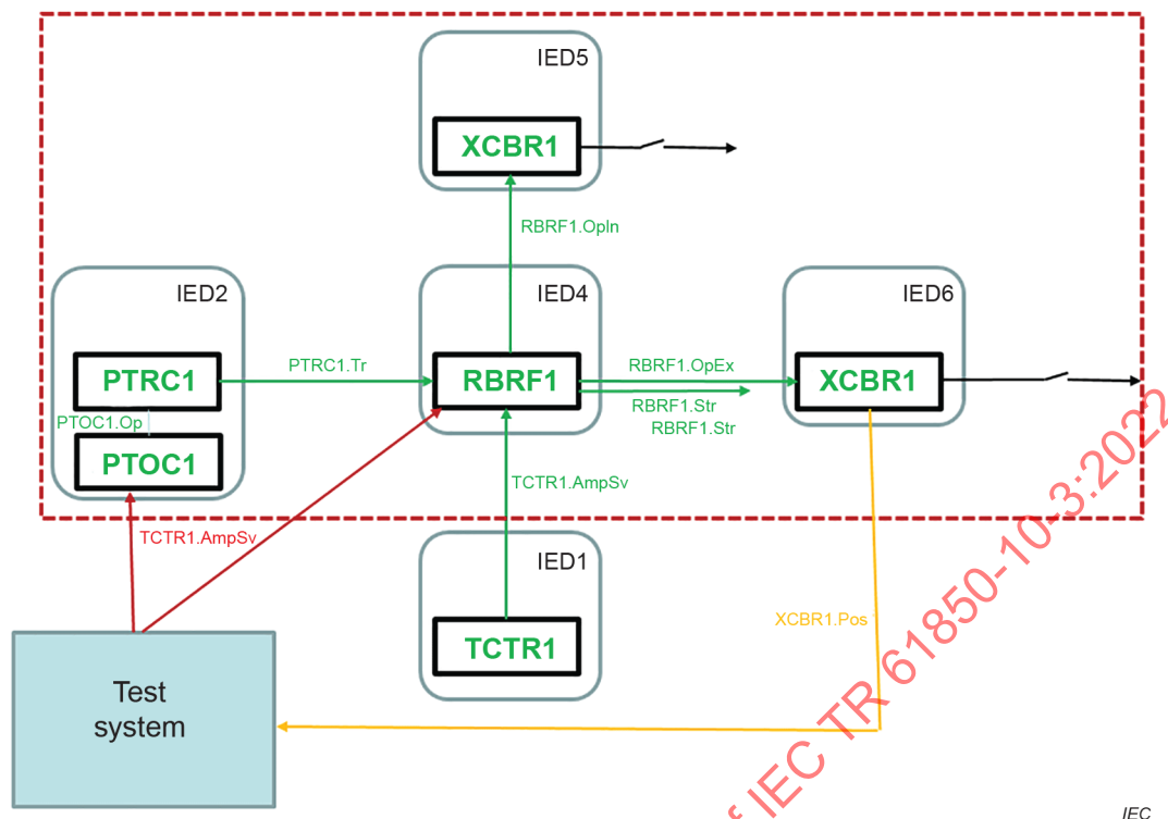
Figure 36 – Interfaces between test system and tested IEDs for End-to-End testing of breaker failure protection scheme
