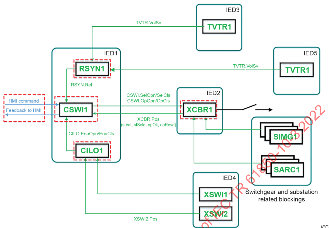
Figure 17 – Select Before Operate Scheme
