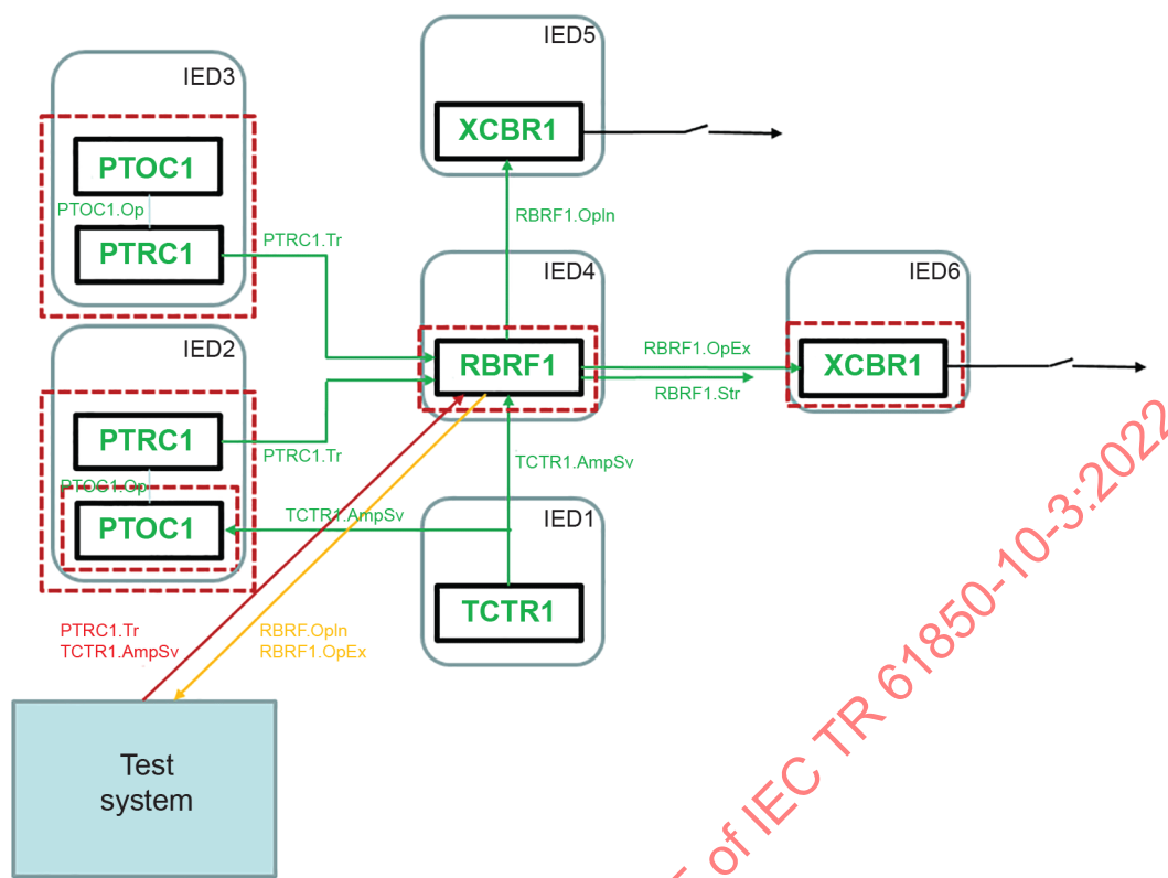
Figure 32 – Interfaces between test system and tested IED for testing of breaker failure protection function
