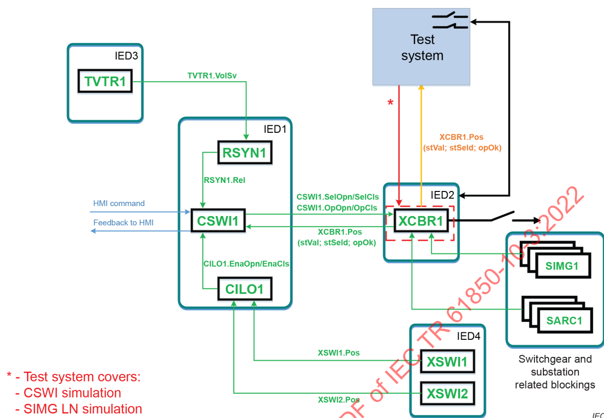
Figure 41 – Unit test of XCBR LN – Scenario 2 – simplified
