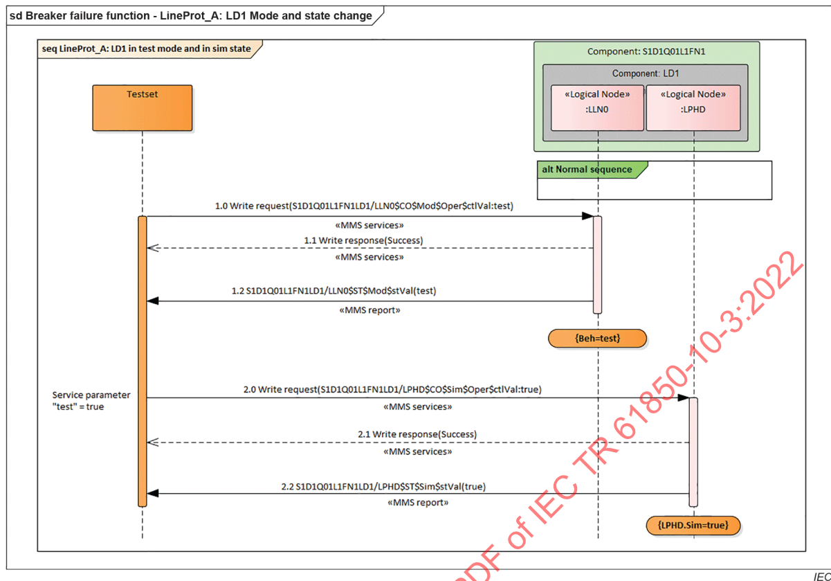
Figure 25 – Line protection function: Setting the mode and the simulation state
