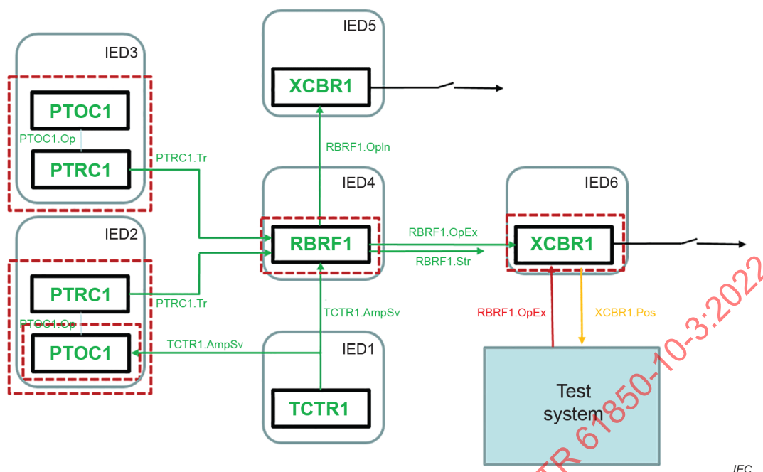
Figure 34 – Interfaces between test system and tested IED for testing of breaker control function
