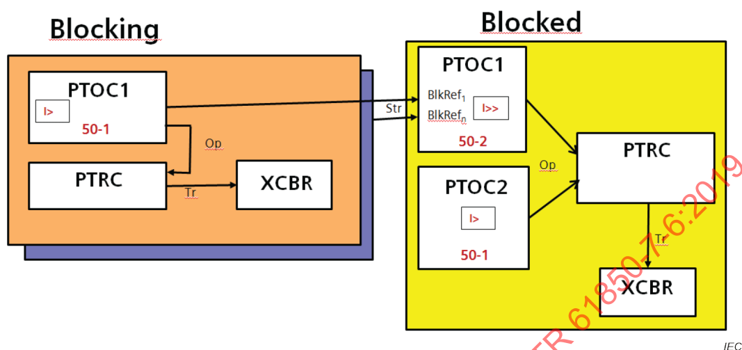
Figure A.6 – Logical architecture reverse blocking
