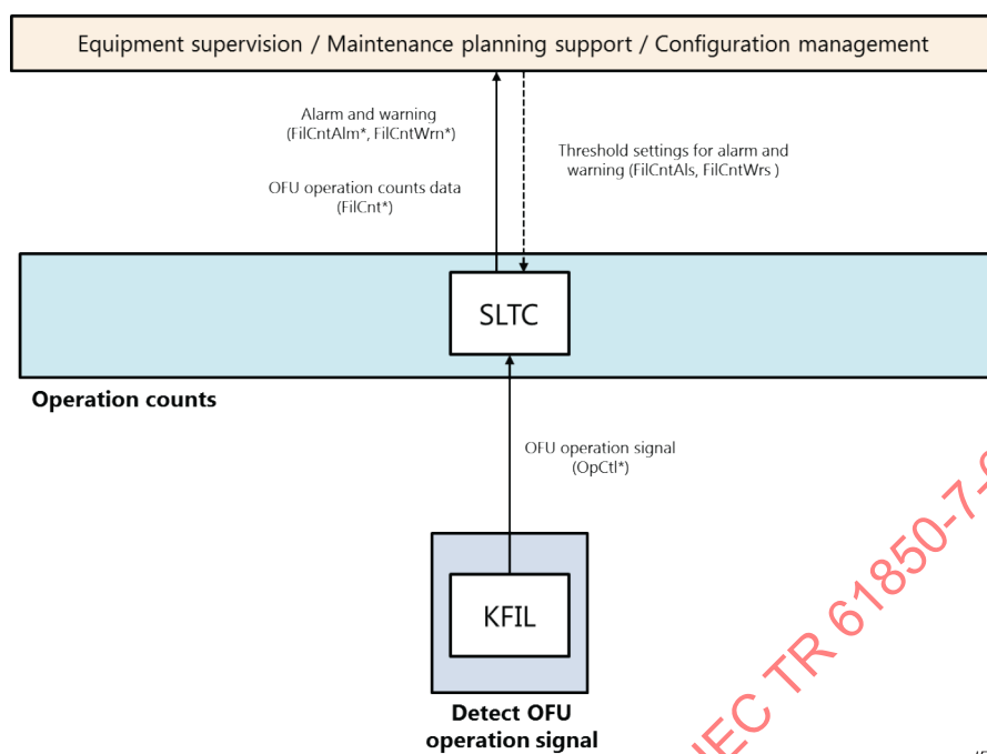
Figure B.15 – Logical architecture for monitoring operation of oil filter unit
