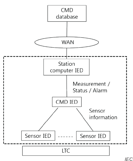
Figure B.3 – Typical system configuration of LTC condition monitoring system
