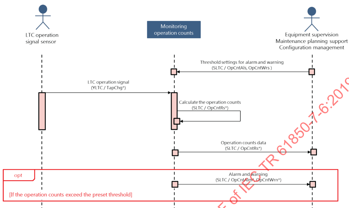
Figure B.6 – Sequence diagram for monitoring operation counts
