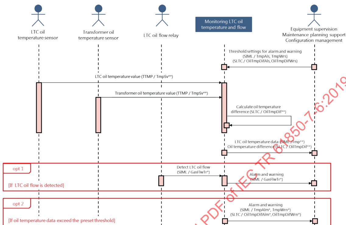
Figure B.8 – Sequence diagram for monitoring oil temperature and flow
