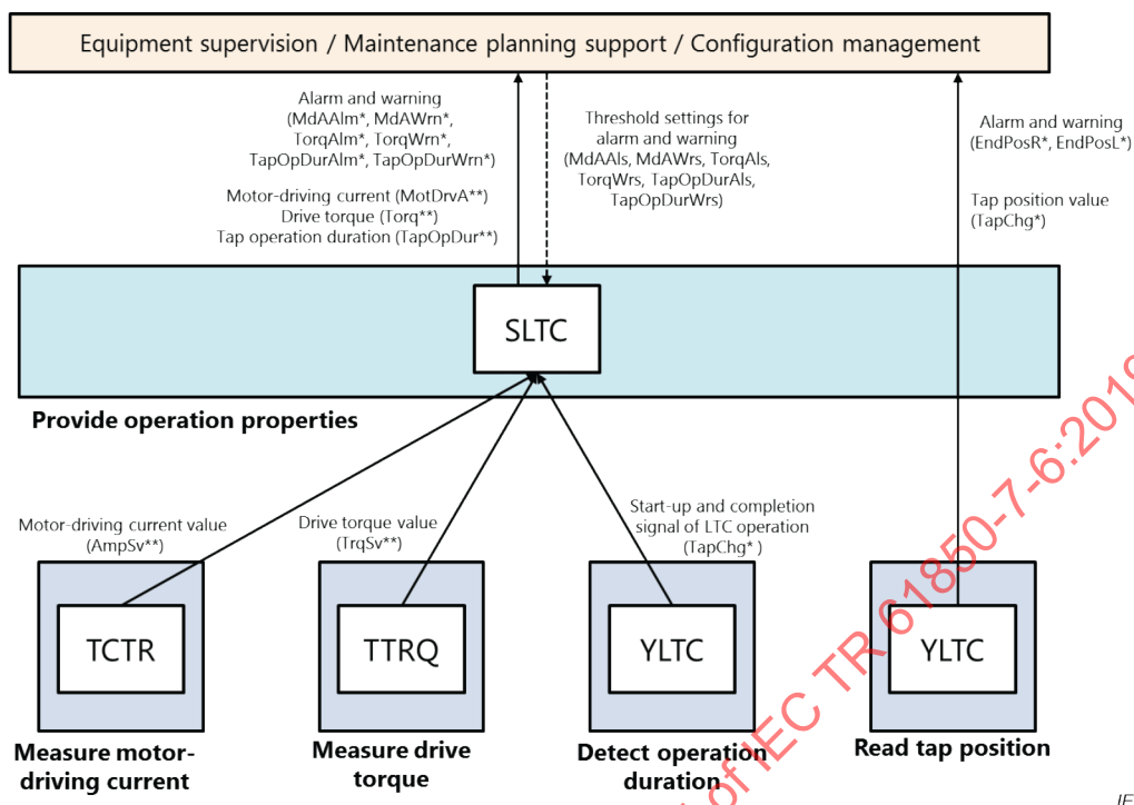
Figure B.11 – Logical architecture for monitoring operation property
