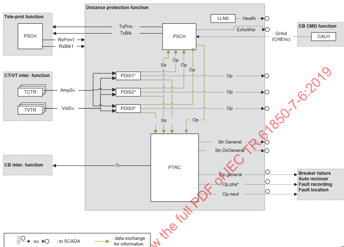
Figure C.3 – Logical architecture distance protection
