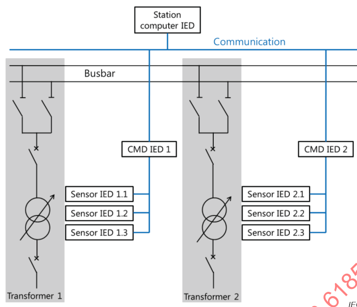
Figure B.2 – Overview of system configuration of LTC condition monitoring
