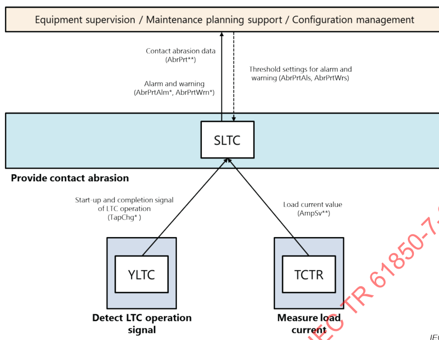
Figure B.13 – Logical architecture for monitoring contact abrasion
