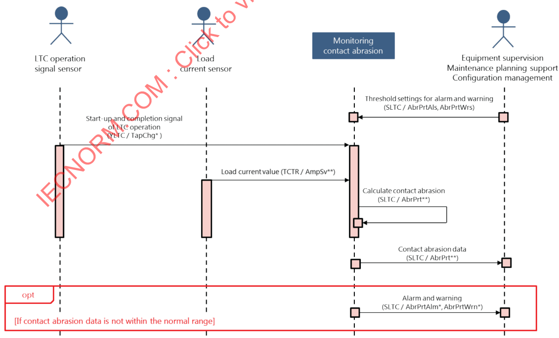
Figure B.7 – Sequence diagram for monitoring contact abrasion
