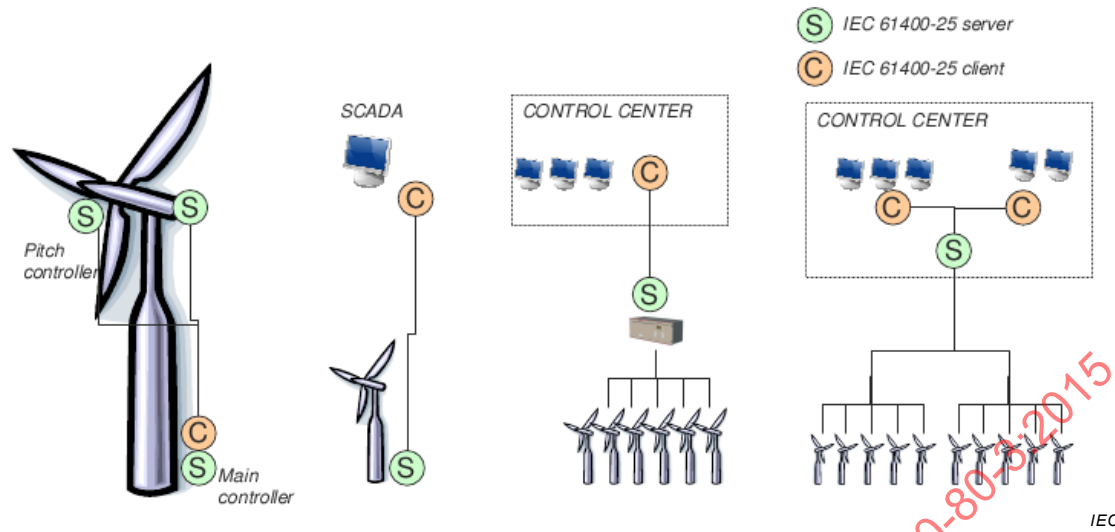
Figure A.5 – Examples of the variety of topologies required/supported for wind power
