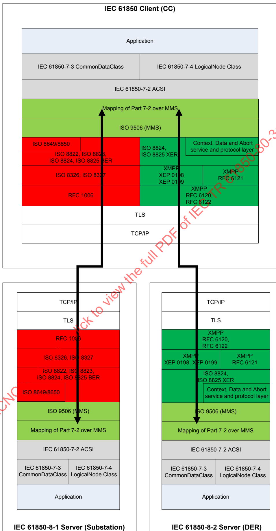
Figure 17 – Control center with dual stack SCSM 8-1 / SCSM 8-2
