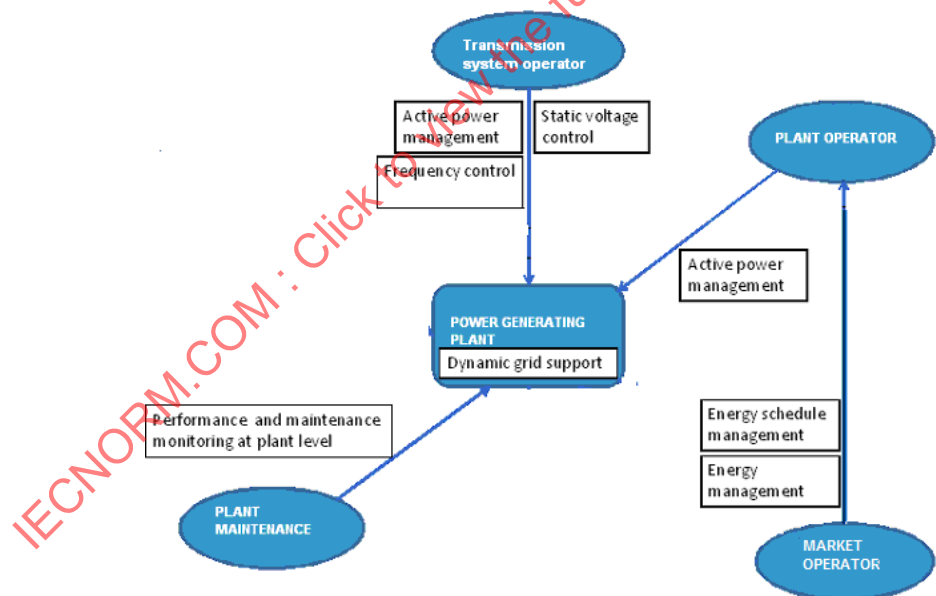
Figure A.4 – Power plants – Relationship between the actors
