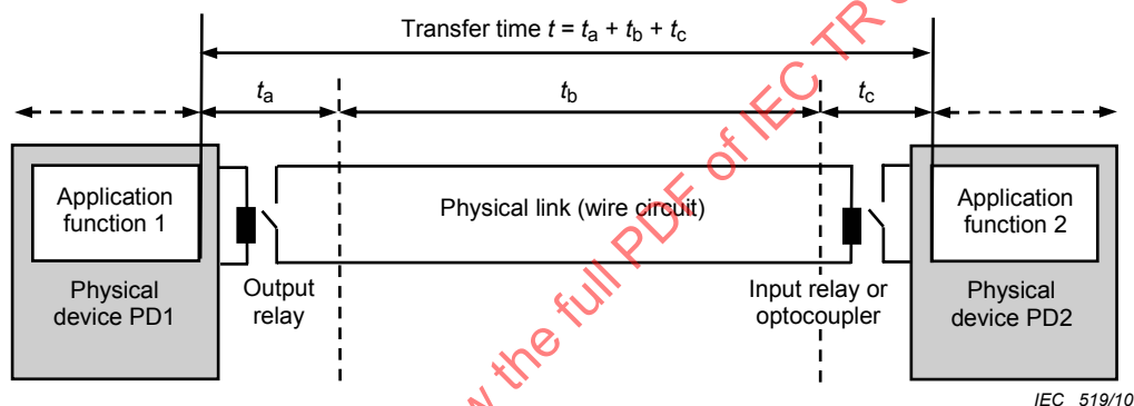
Figure 16 – Transfer time for binary signal with conventional output and input relays
