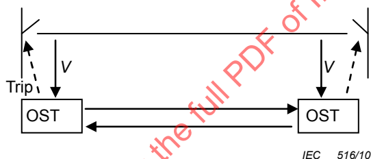
Figure 13 – Out-of-step detection
