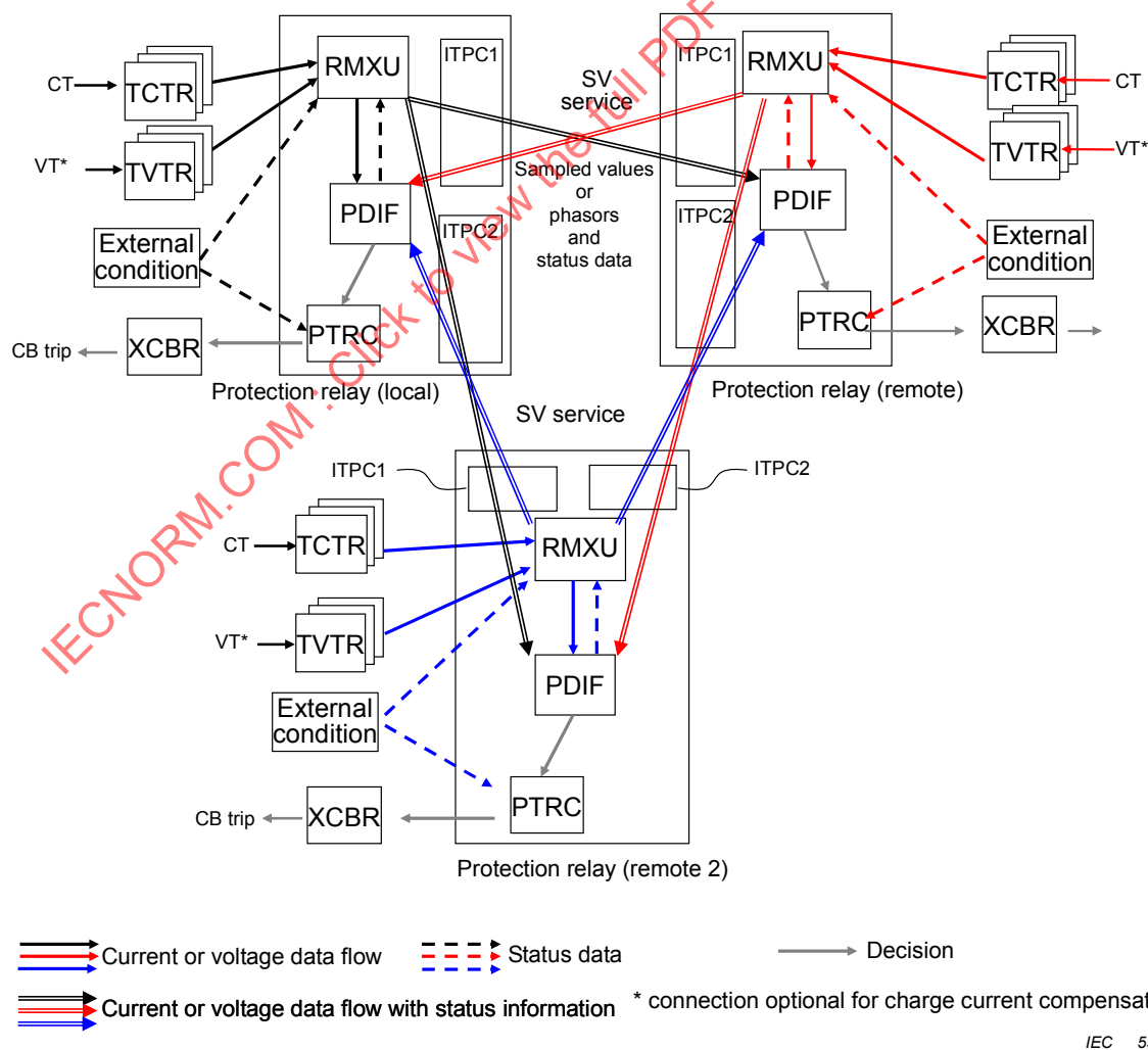
Figure 27 – Proposed 3-terminal current differential feeder protection relay model
