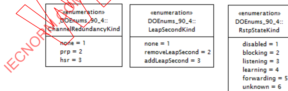
Figure 84 – Class diagram DetailedDiagram::DOEnums_90_4
