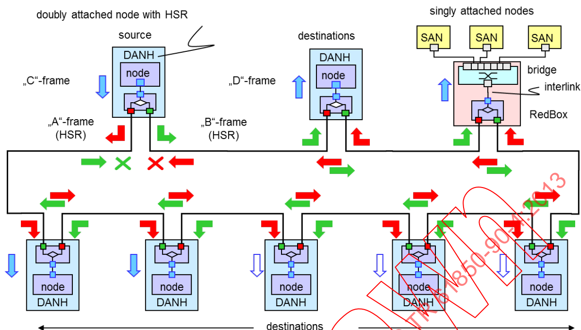
Figure 21 – HSR principle
