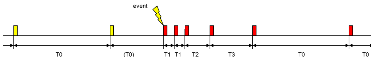
Figure 9 – GOOSE protocol time chart
