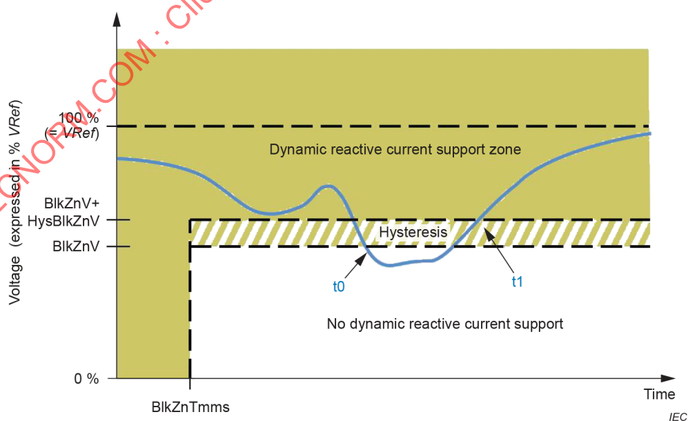
Figure 28 – Settings to define a blocking zone
