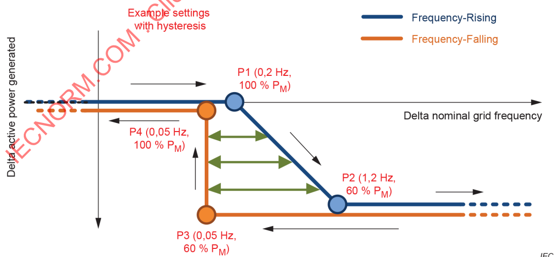
Figure 19 – Frequency-based active power modification with the use of an array
