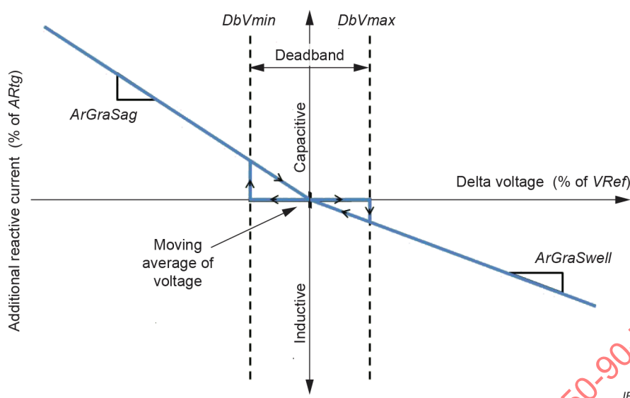
Figure 27 – Alternative gradient behaviour, selected by ArGraMod
