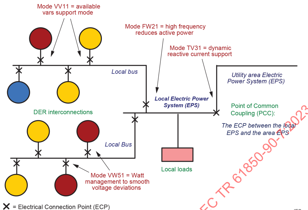
Figure 7 – Example of modes associated with different ECPs
