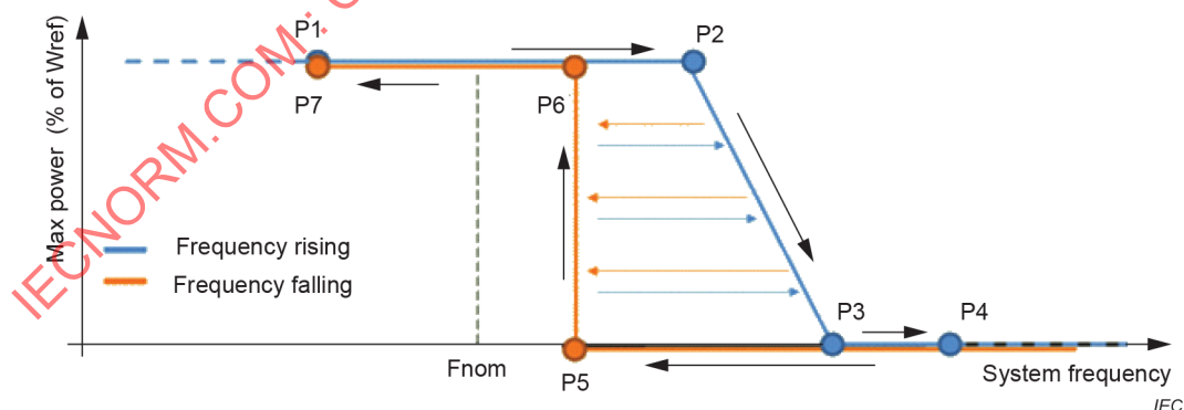
Figure 22 – Example of an asymmetrical hysteresis configuration
