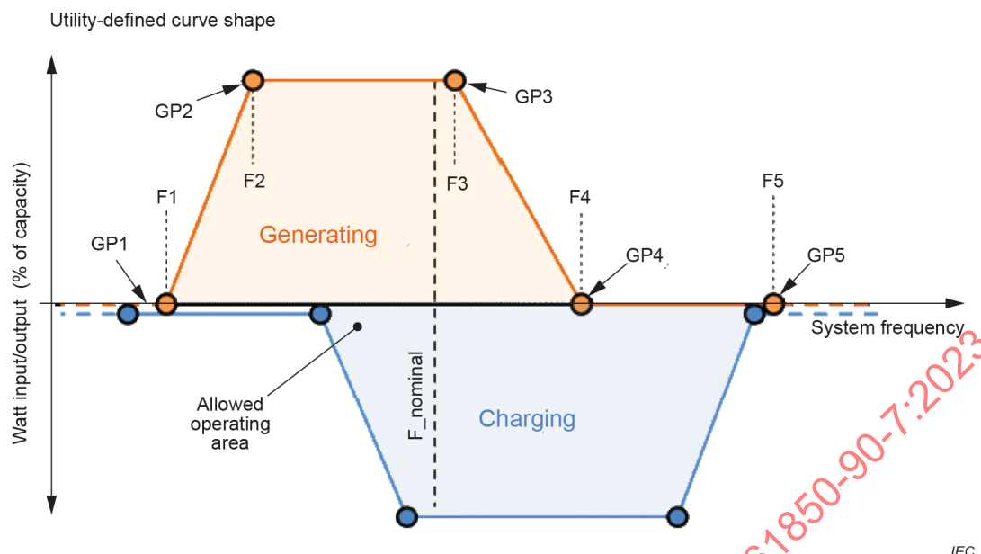
Figure 17 – Frequency-watt mode curves
