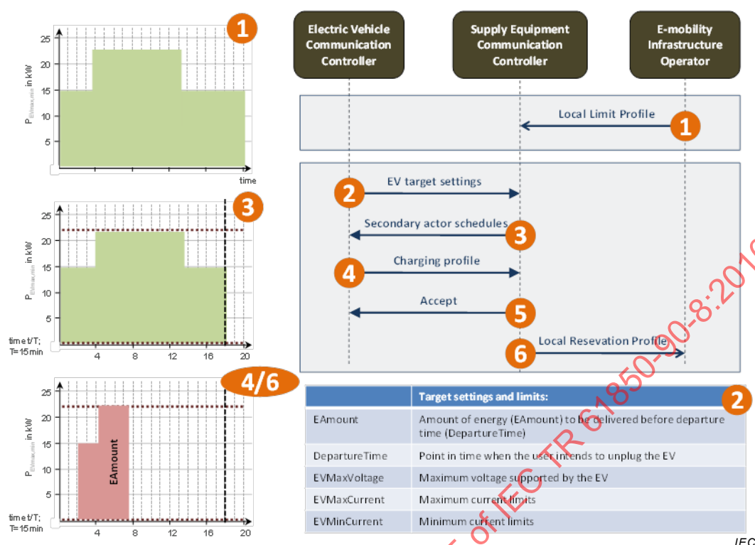
Figure 8 – Exemplary exchange of charge schedule information for an EVSE with one outlet, based on [IEEE VPPC2011]
