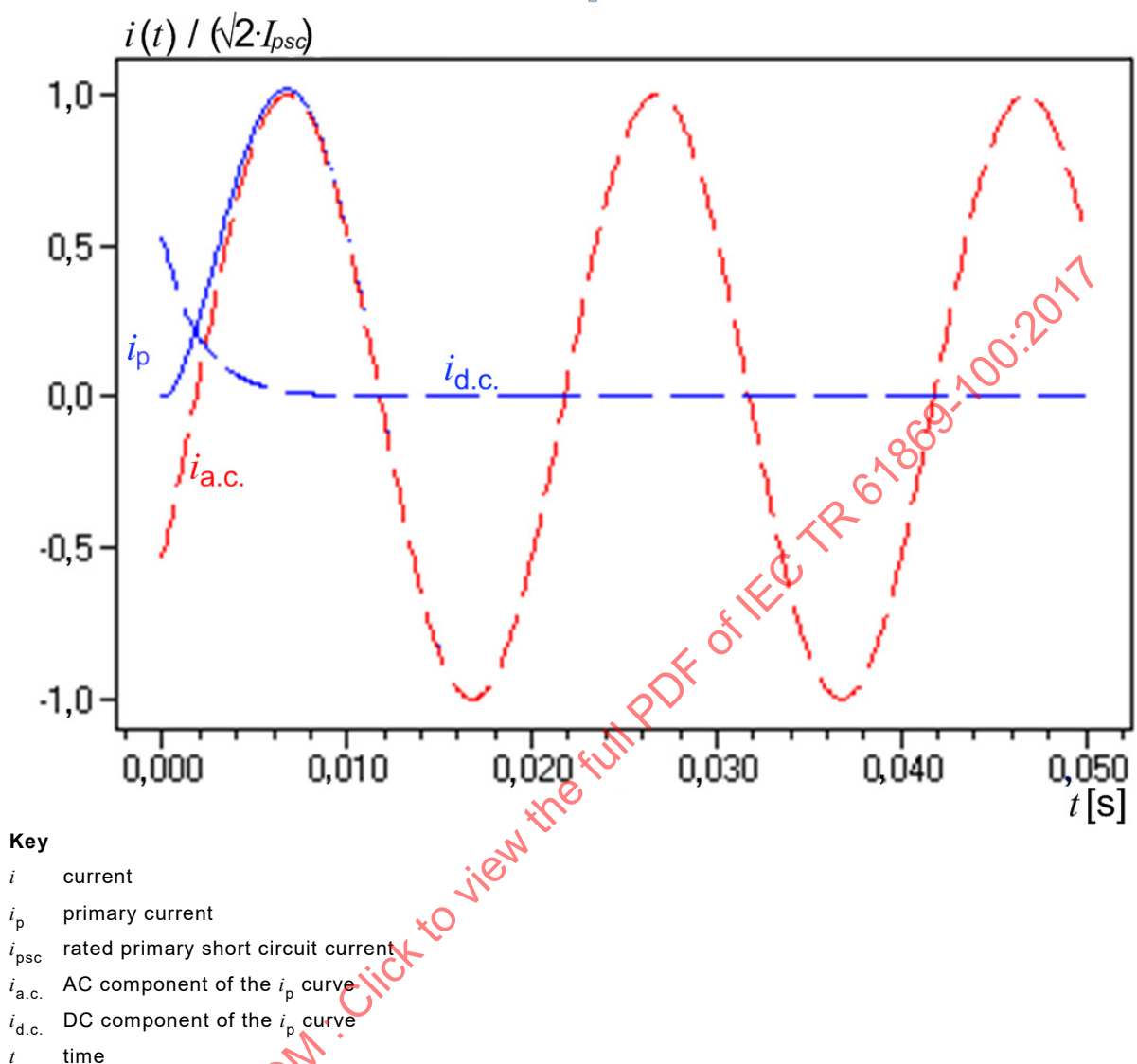
Figure 26 – Primary current for a short primary time constant
