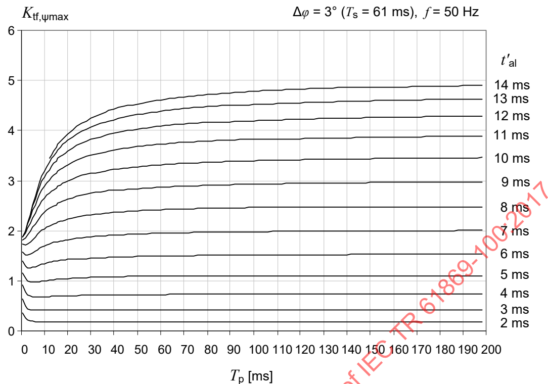
a) T_s = 61 ms at 50 Hz
