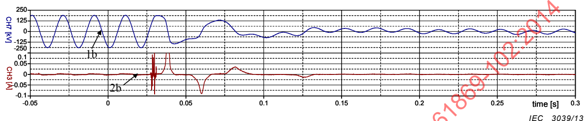
b) Non-steady state, decreasing ferroresonance oscillation, transient waveform (between 0,03 and 0,15 s); switching near zero crossing of voltage (between 0,15 s and 0,3 s the coupled a.c. voltage can be seen)
