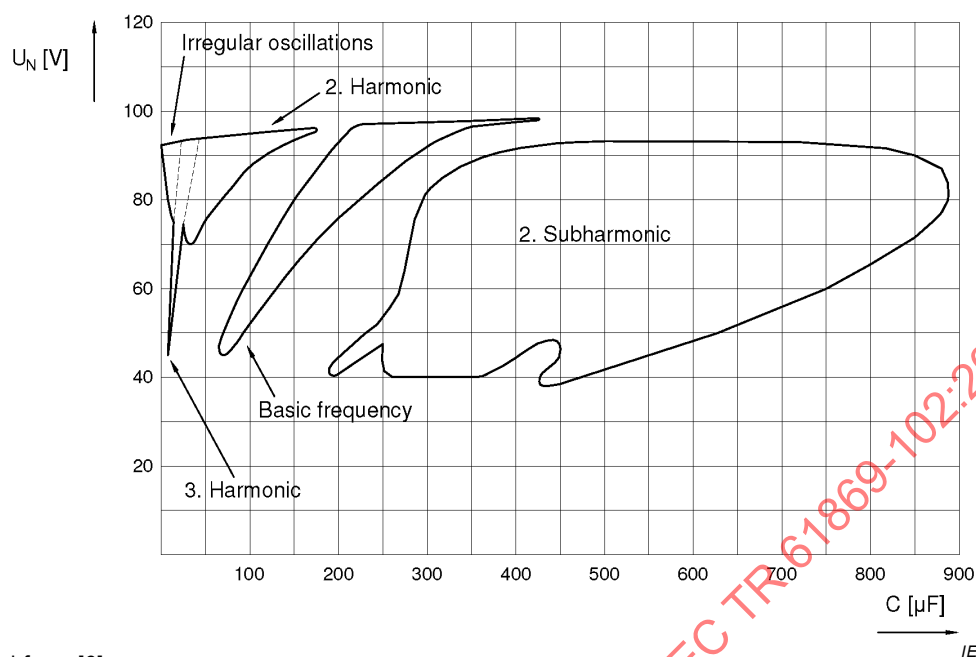
Figure 10 – Domains in the capacitance C and line voltage U where different harmonic and sub-harmonic ferroresonance oscillations are obtained for a given resistance R of 6,7 \Omega in Bergmann's test set
