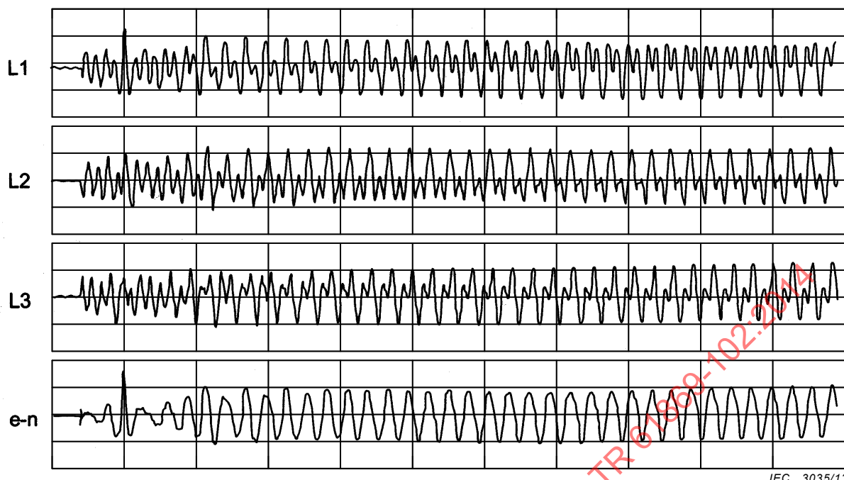
Figure 13 – Fault recorder display of a three-phase ferroresonance oscillation
