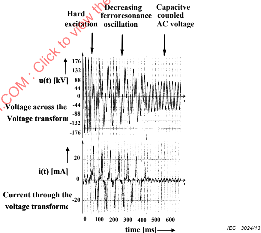
b) Single-phase decreasing ferroresonance oscillations, type 2c according to Table 1
