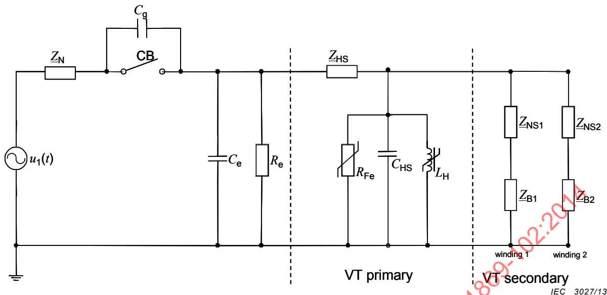
a) Excitation of ferroresonance oscillation through a grading capacitor
