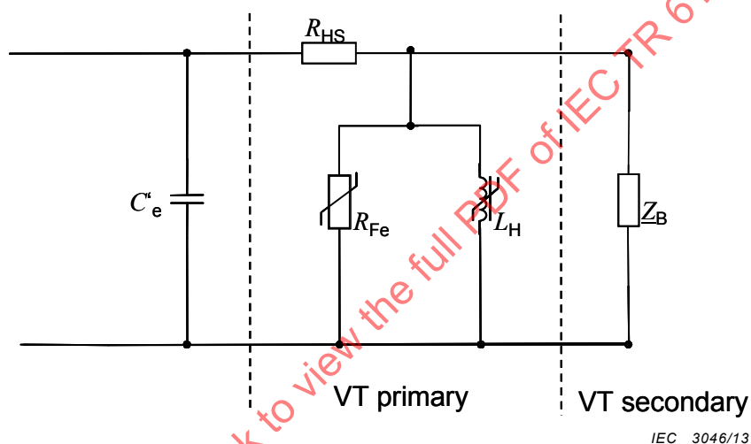
b) Simplified VT-circuit for ferroresonance studies
