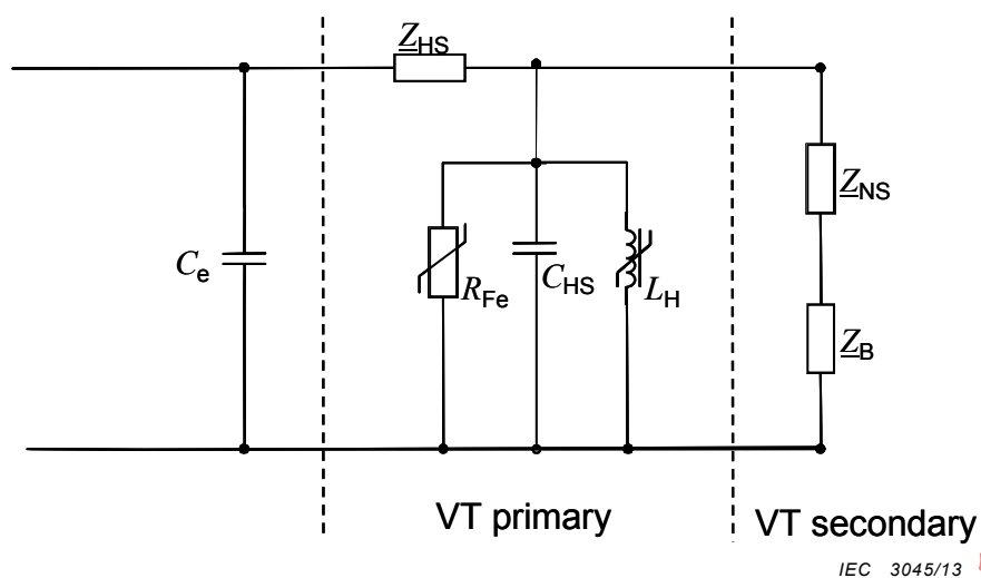
a) VT-schematic circuit
