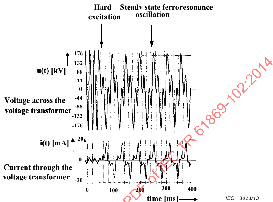
a) Single-phase steady state ferroresonance oscillations, type 2a according to Table 1
