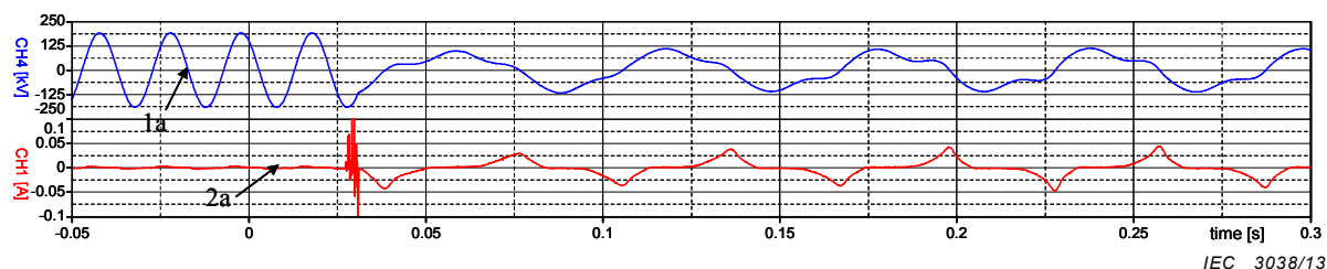
a) Steady state ferroresonance oscillations, frequency 16^{2/3} Hz; switching near the voltage maximum
