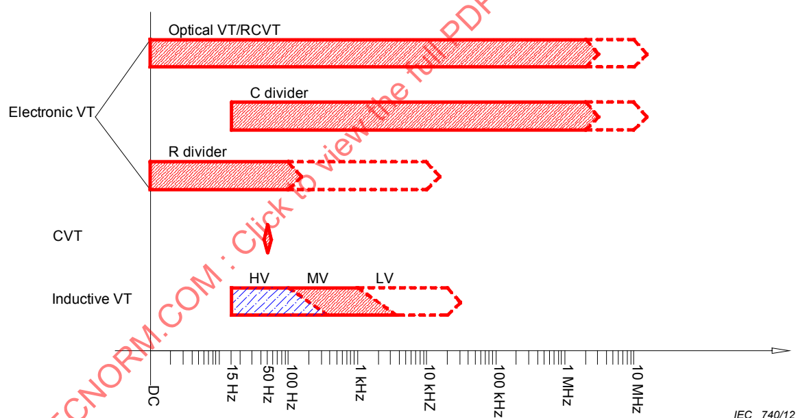
Figure 9 – Voltage transformer technologies frequency range according to present experience
