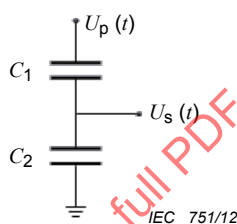
Figure 35 – Electrical scheme of a capacitive voltage divider
