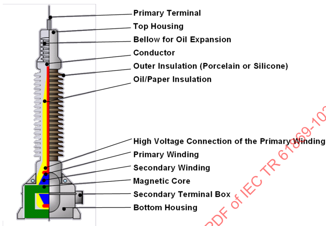
Figure 13 – Cross-section view of a freestanding High Voltage VT (courtesy of Trench Switzerland AG)
