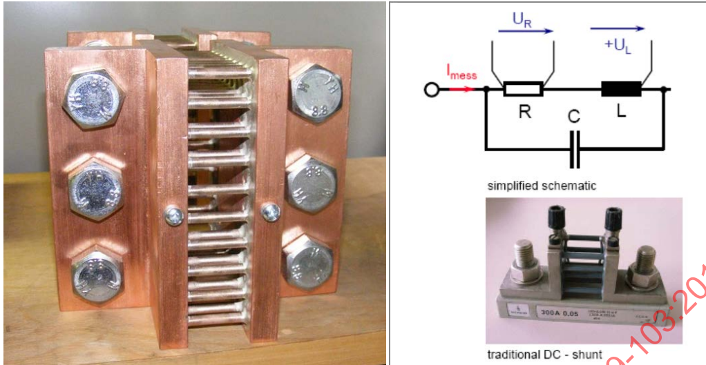
Figure 47 – Shunt for DC application (Courtesy of Alstom Grid)
