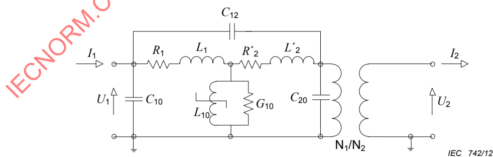
Figure 11 – Example of equivalent circuit for an inductive voltage/current transformer
