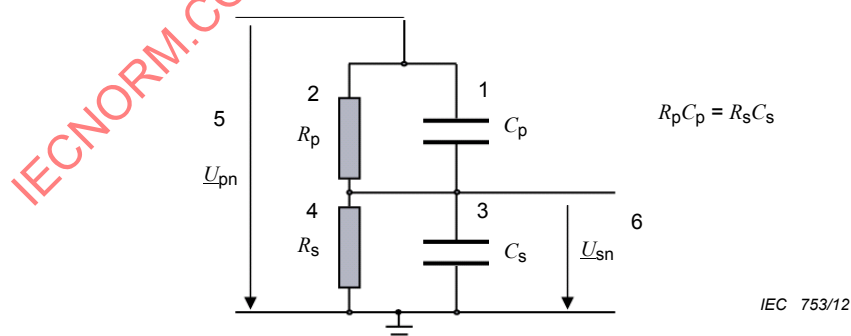
Figure 37 – Equivalent circuit of a balanced RC voltage divider (from x))
