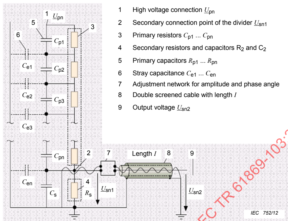
Figure 36 – Equivalent circuit of an RC voltage divider (from w), x))
