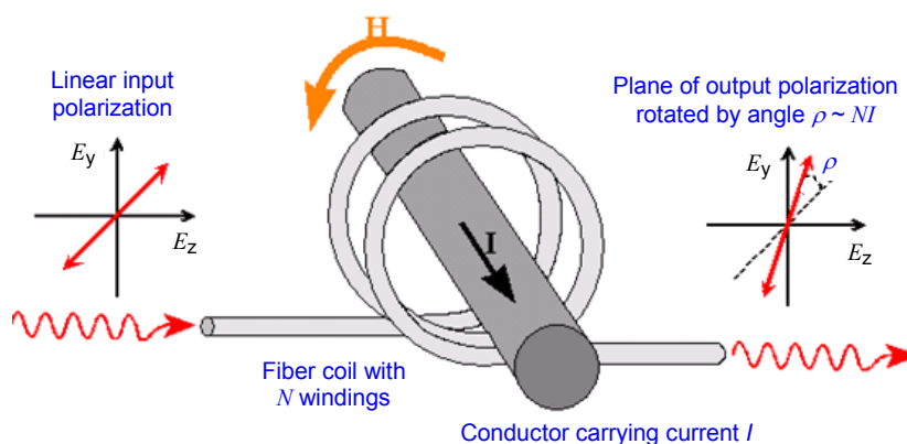
Figure 40 – Principle of optical CT measurement (from v))
