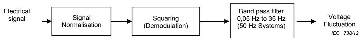
Figure 4 – Demodulation within the IEC flickermeter
