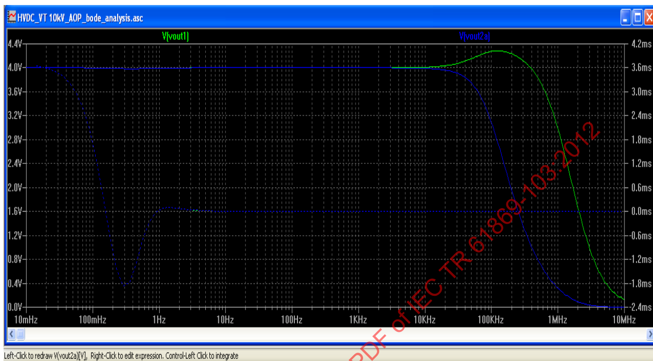
Figure 31 – Frequency response calculation for an optical VT (courtesy of Alstom Grid)
