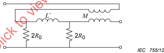
Figure 48 – Equivalent circuit for a compensated shunt
