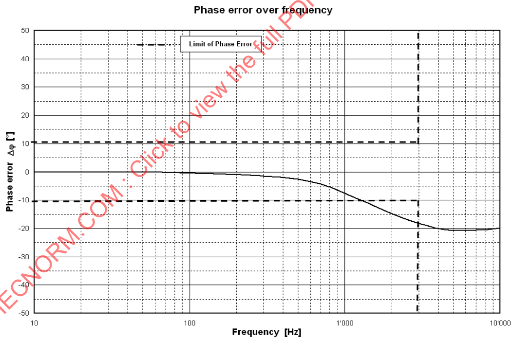
Figure 34 – Phase error of MV resistive divider (courtesy of Trench Switzerland AG)
