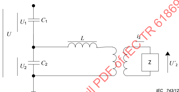
Figure 20 – CVT: Equivalent circuit at power frequency
