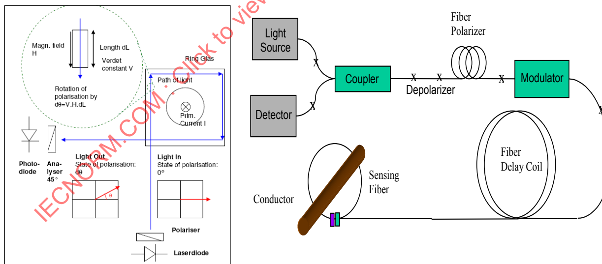
Figure 41 – Principle of optical CT measurement (Courtesy of Alstom Grid)
