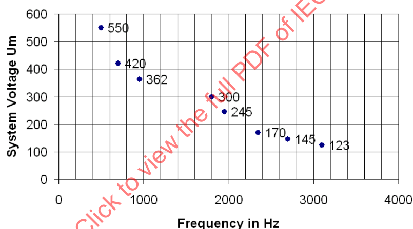
Figure 15 – First resonance peak depending on the system voltage U_m (courtesy of Trench Switzerland AG)
