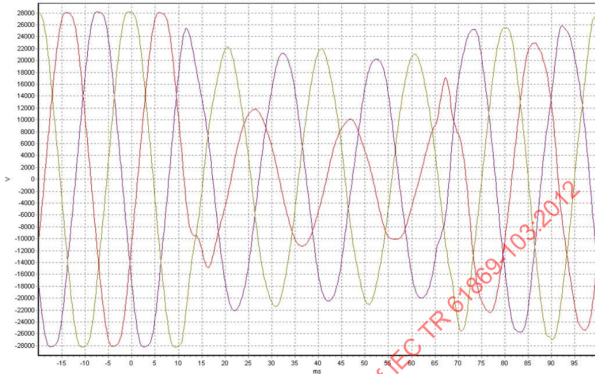
Figure 5 – Example of voltage dip (courtesy of Italian distribution network monitoring system – QuEEN)
