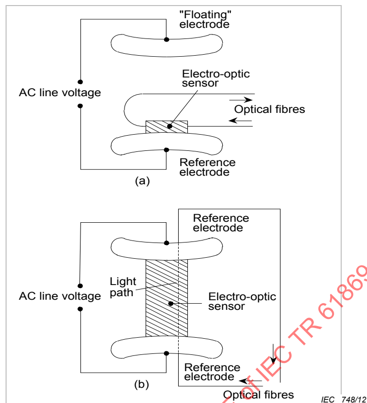
Figure 27 – Various solutions to apply voltage on the active crystal
