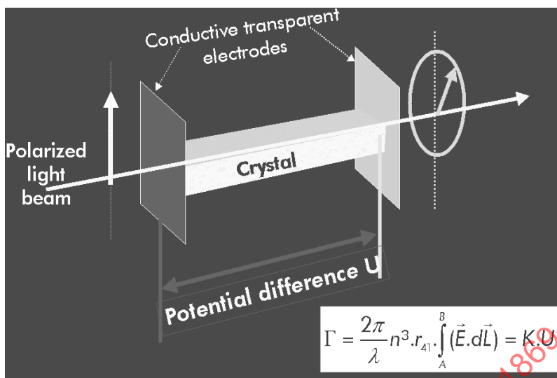
Figure 26 – Basic design for a bulk crystal producing a Pockels Effect (courtesy of Alstom Grid)
