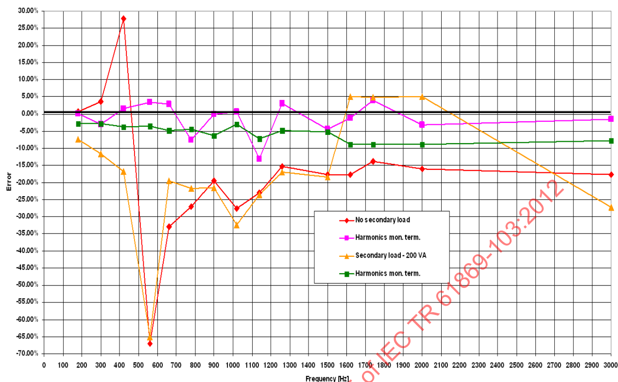
Figure 25 – Comparison of different measurements with and without harmonic monitoring terminal (Courtesy of Trench Switzerland AG, based on p))
