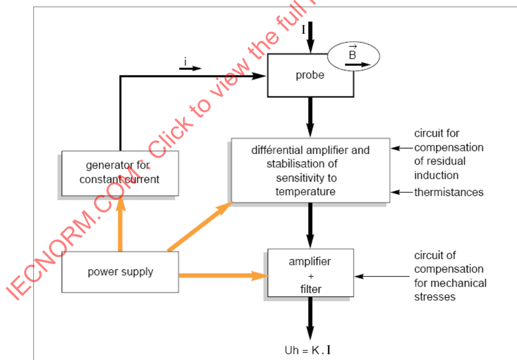
Figure 52 – Hall Effect Sensor (Courtesy of Schneider Electric – From II)
