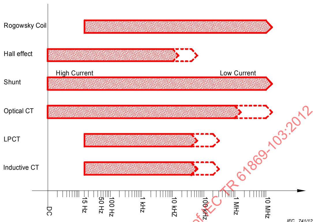
Figure 10 – Current transformer technologies frequency range according to present experience
