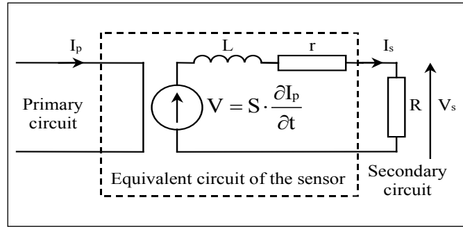
Figure 44 – Equivalent circuit for a Rogowski coils (Courtesy of Alstom Grid))
