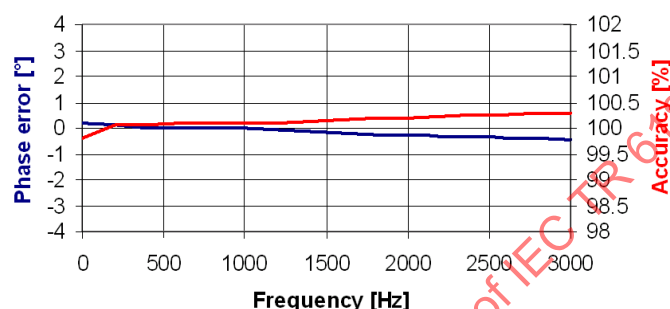
Figure 38 – Frequency response of an RC voltage divider (courtesy of Trench Switzerland AG)
