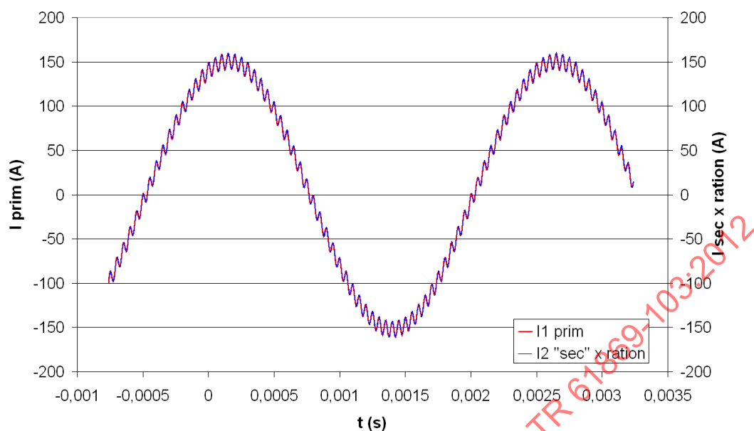
Figure 17 – Results obtained for a 245 kV CT (courtesy of Trench Switzerland AG)
