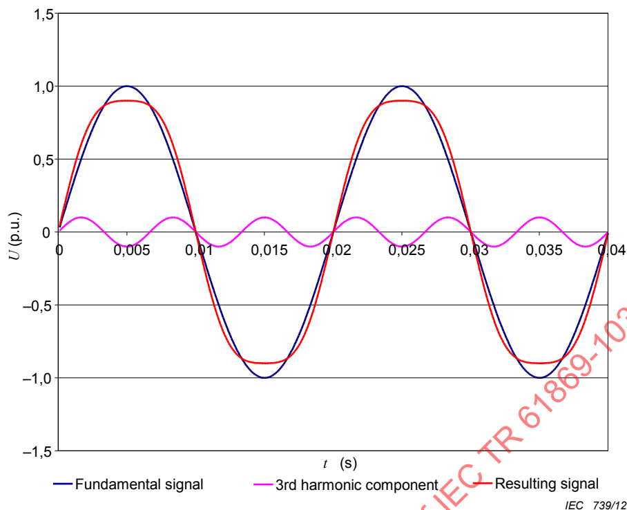
Figure 8 – Example of voltage harmonics
