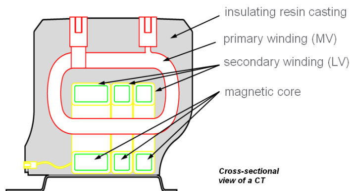
Figure 16 – Cross-section view of a current transformer (courtesy of Schneider Electric)
