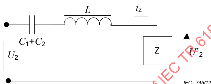
Figure 22 – Simplified CVT Thevenin equivalent circuit at power frequency
