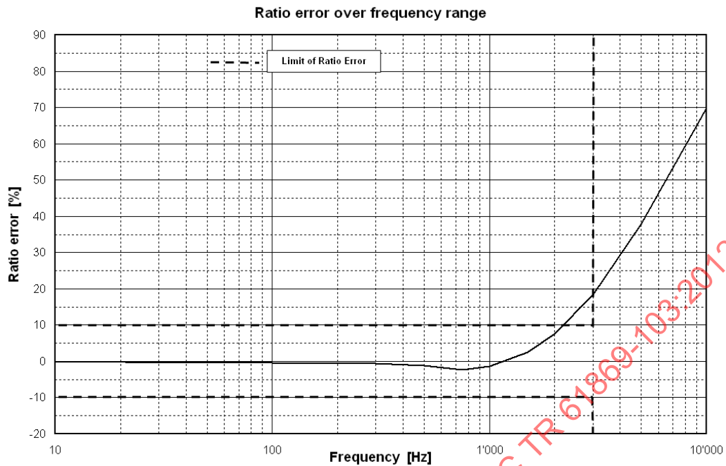
Figure 33 – Ratio error of an MV resistive divider (courtesy of Trench Switzerland AG)
