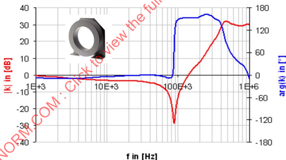
Figure 43 – Typical frequency response measurement of a LPCT (Courtesy of Trench Switzerland AG)
