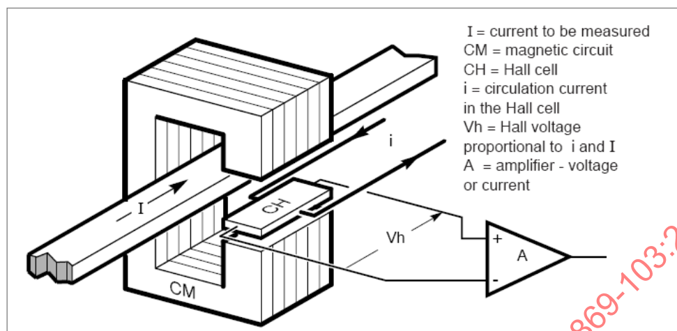
Figure 51 – Hall Effect Sensor (Courtesy of Schneider Electric – From II)
