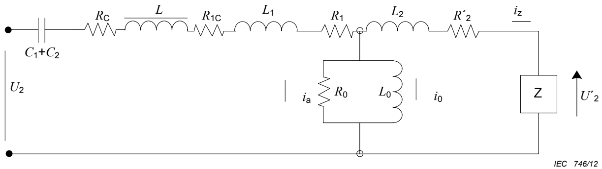
Figure 23 – Complete CVT Thevenin equivalent circuit at power frequency
