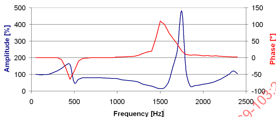
Figure 14 – Frequency response of a typical inductive VT 420 kV (courtesy of Trench Switzerland AG)
