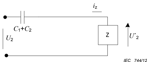
Figure 21 – Simplified CVT Thevenin equivalent circuit at power frequency without compensating reactor
