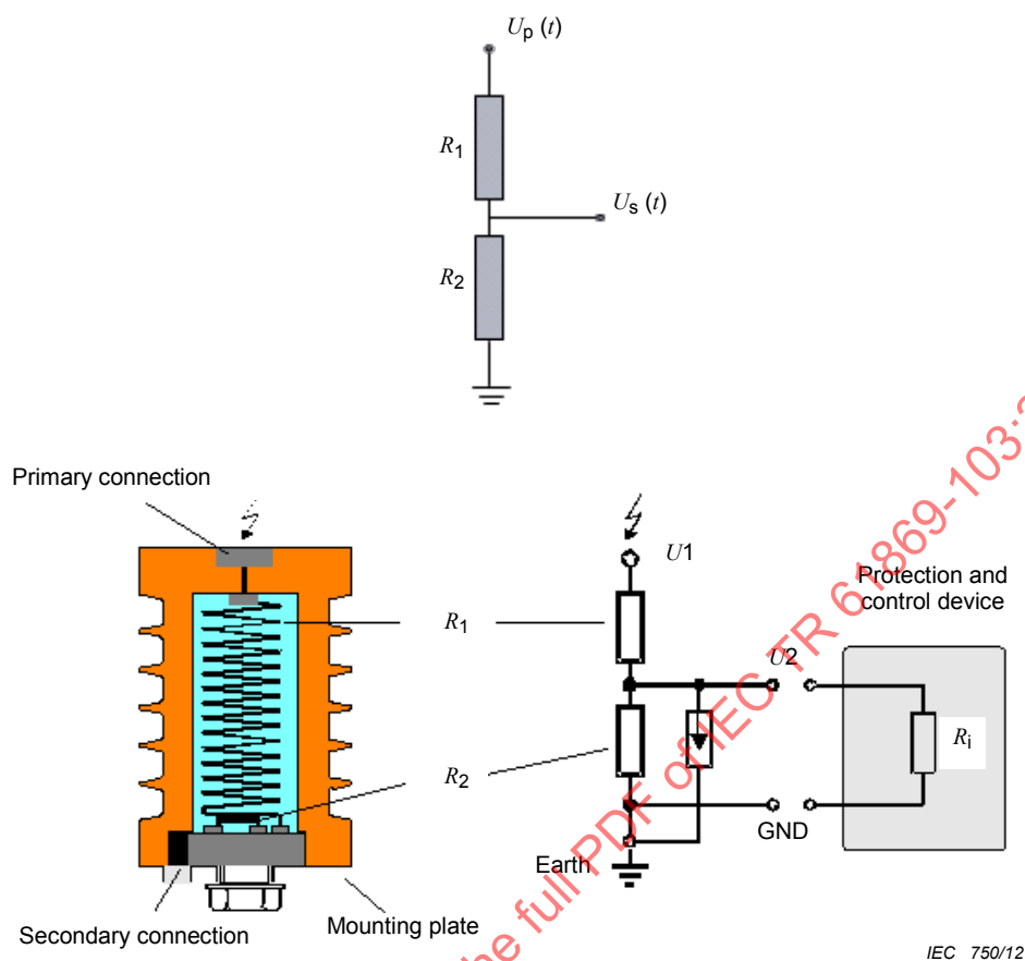
Figure 32 – Cross section view and electrical scheme of a resistive voltage divider (from v))
