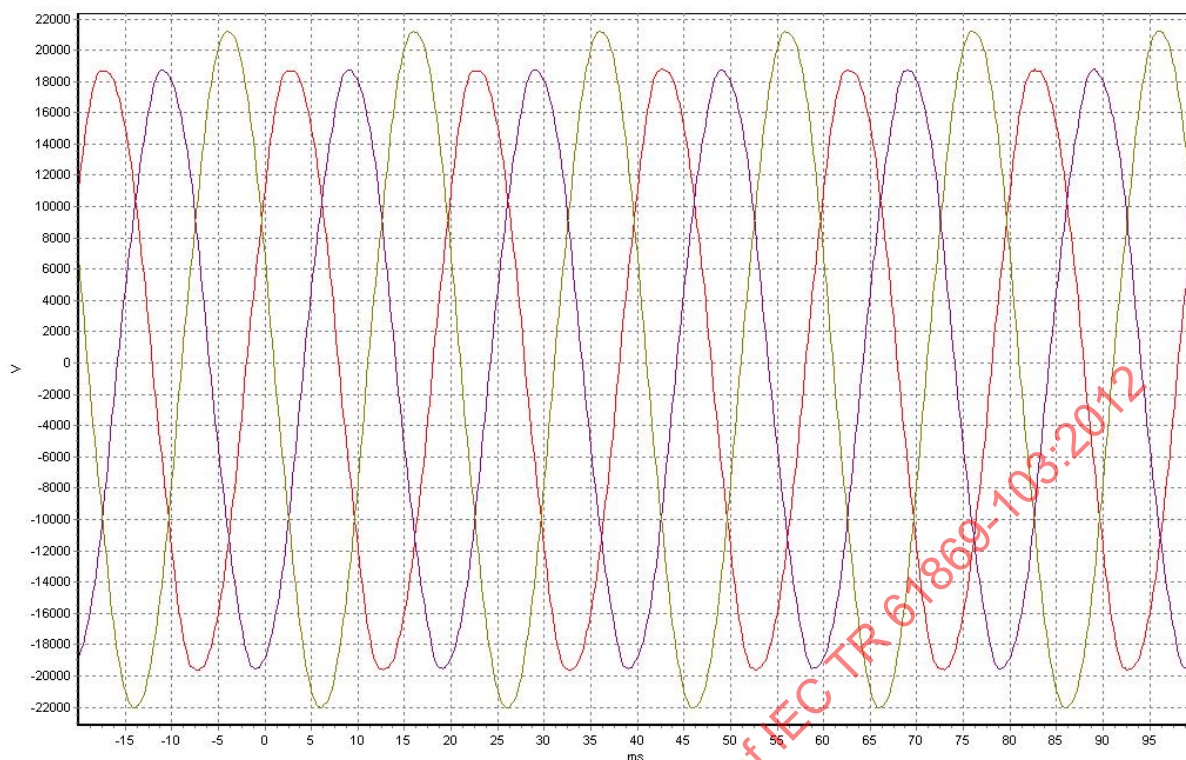
Figure 7 – Example of voltage unbalance (courtesy of Italian distribution network monitoring system- QuEEN)
