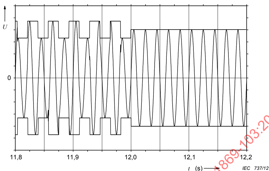
Figure 3 – Example of voltage fluctuation causing flicker
