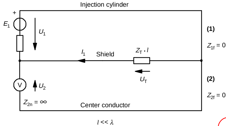
Figure 3a – Equivalent circuit for the definition and possible testing of Z
