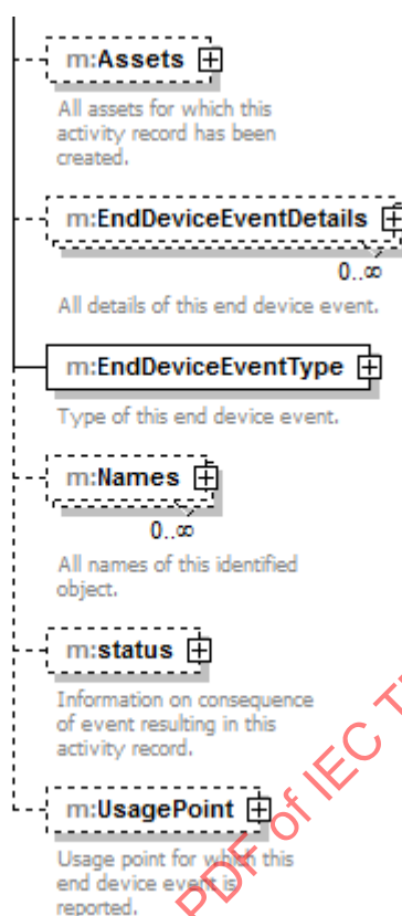
Figure 49 – EndDeviceEvent definition
