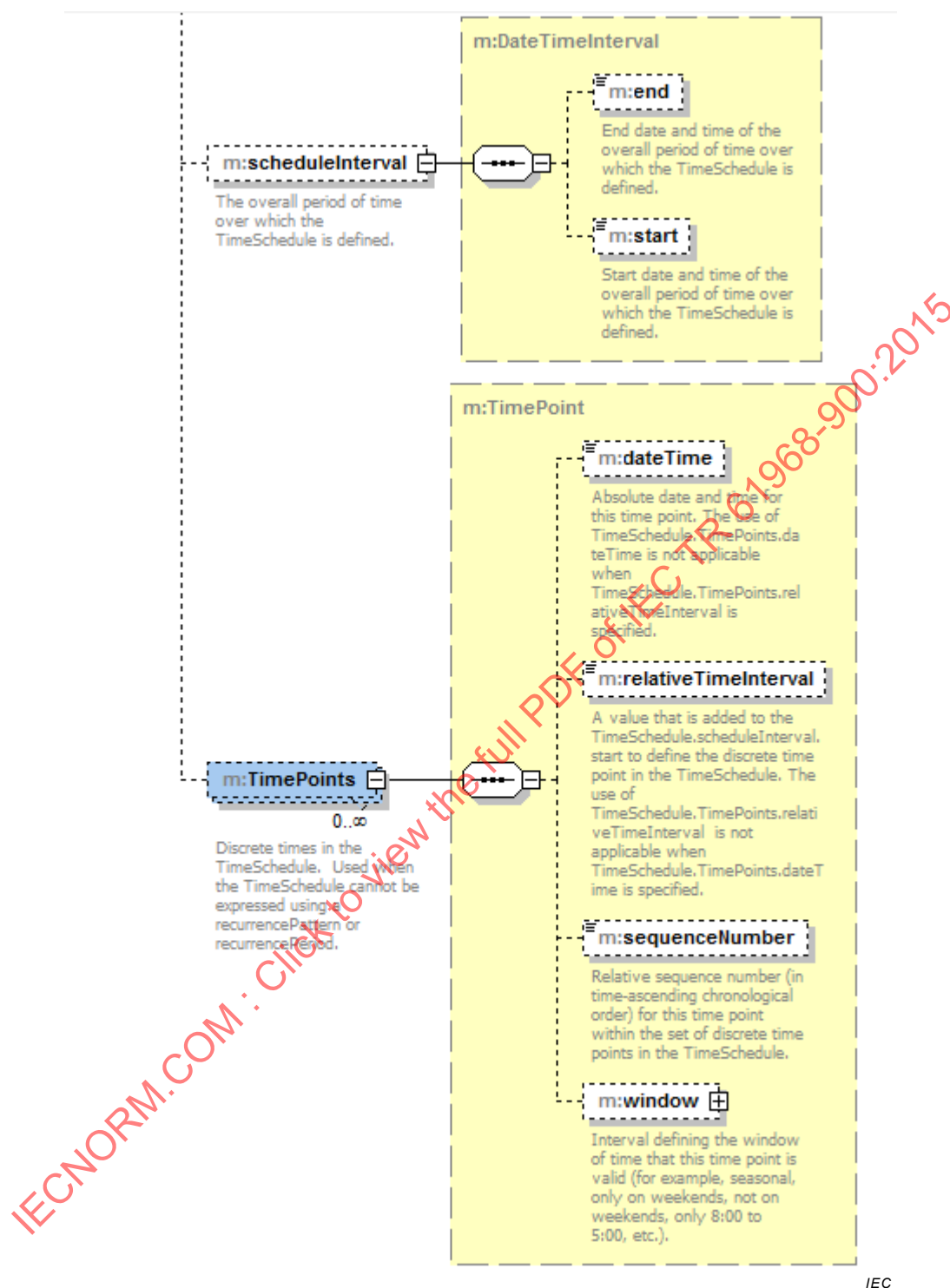
Figure 64 – MeterReadSchedule.TimeSchedule definition
