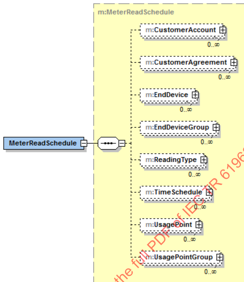
Figure 63 – MeterReadSchedule definition
