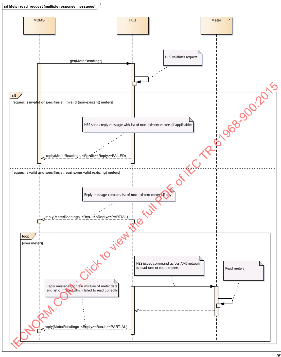
Figure 17 – Message exchange pattern for a meter read request with multiple response messages
