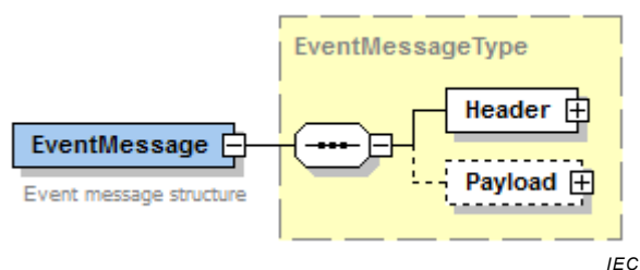
Figure 6 – EventMessage definition according to Message.xsd
