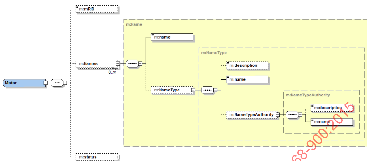
Figure 28 – <MeterReadings><Meter> definition
