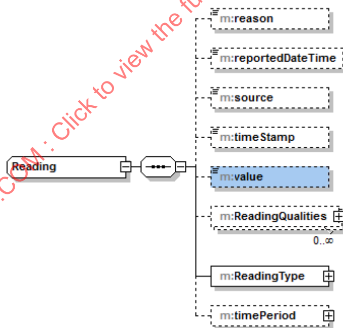
Figure 29 – <MeterReadings><Reading> definition
