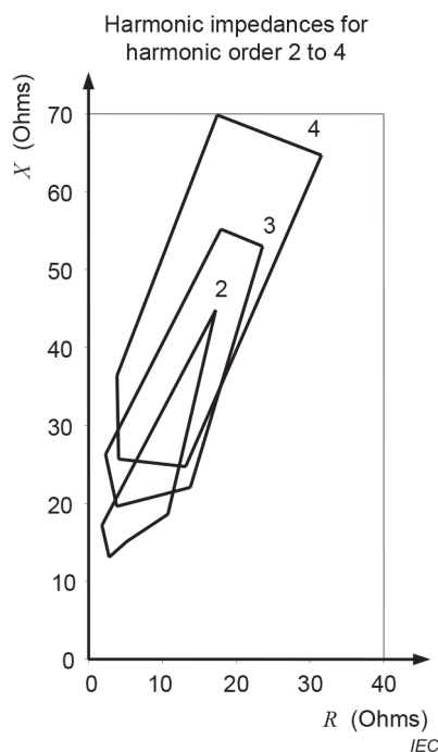
Figure 16 – Example of harmonic impedances for harmonics of order 2 to 4
