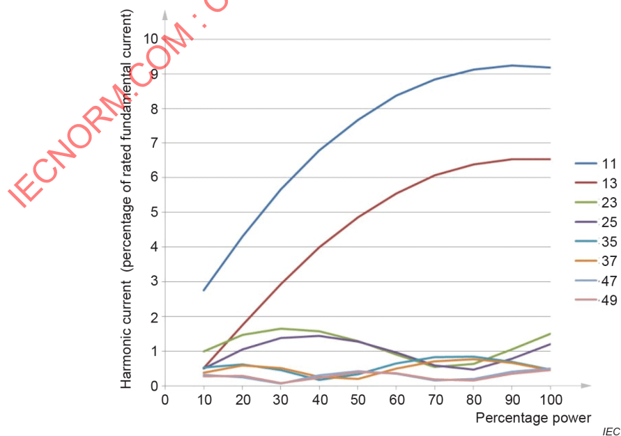
Figure 4 – Typical variation of characteristic harmonic magnitude with direct current
