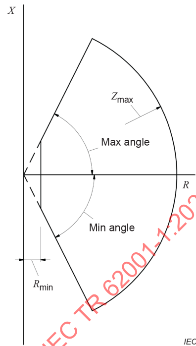
Figure 14 – AC system impedance general sector diagram, with minimum resistance
