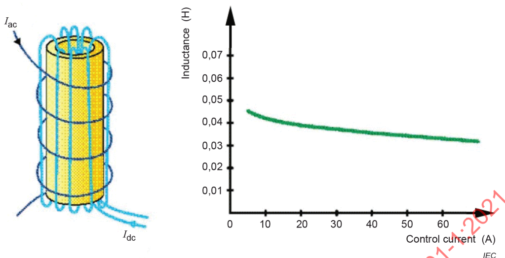
Figure 25 – Design principle of a self-tuned reactor using DC control current in an orthogonal winding
