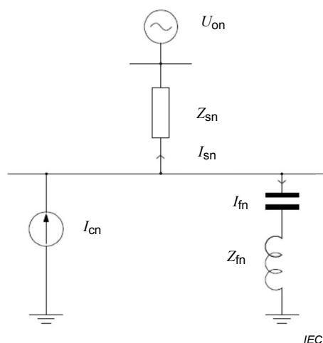
Figure 26 – Circuit for rating evaluation
