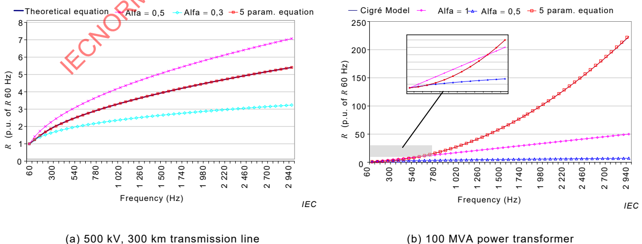
Figure B.8 – Comparison of different approximations for resistance variations
