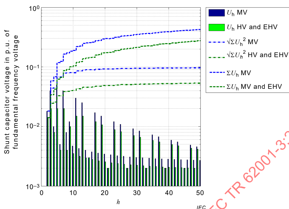
Figure 25 – Harmonic voltage stress on a shunt capacitor with IEC planning levels applied
