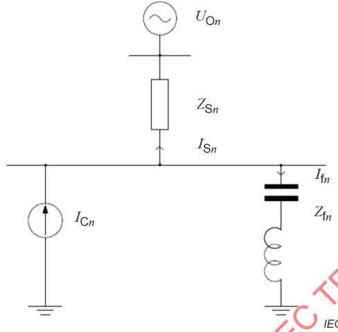
Figure 1 – Circuit for rating evaluation
