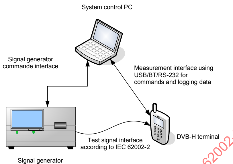
Figure 1 – Example of a test set up in test system controlled measurement
