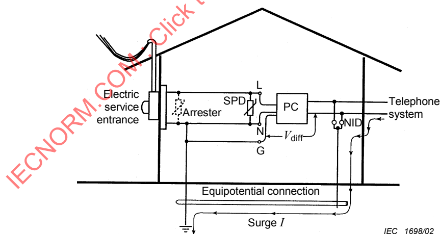
Figure D.2 – Voltage difference appearing across PC/modem during surge current flow
