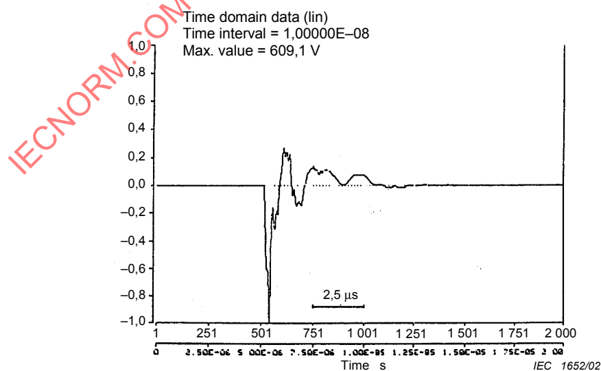
Figure 15 – Example of a high-frequency switching surge
