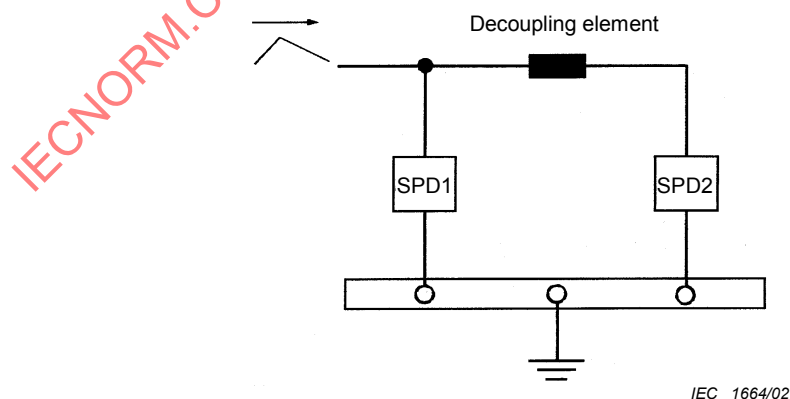
Figure 27 – Basic model for energy coordination of SPDs
