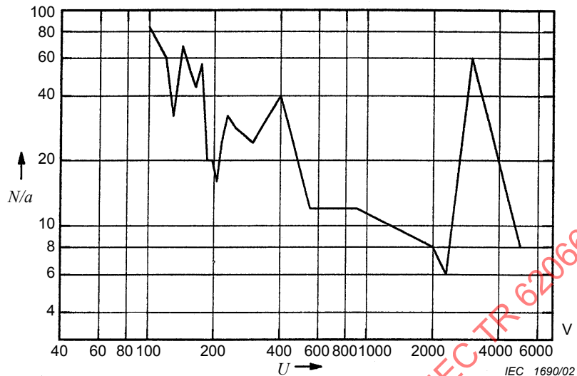
Figure B.7 – Switching surges in an industrial plant measured near the collecting bar
