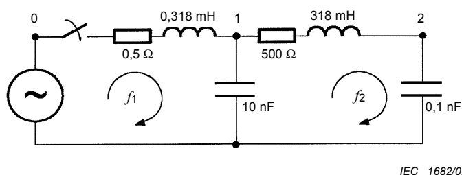
Figure B.1 – Example illustrating transient resonance caused by switching
