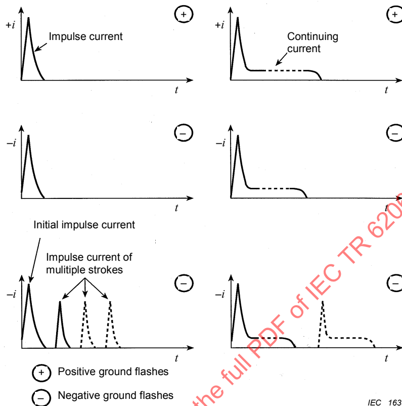
Figure 3 – Possible waveforms of lightning current striking ground-based objects
