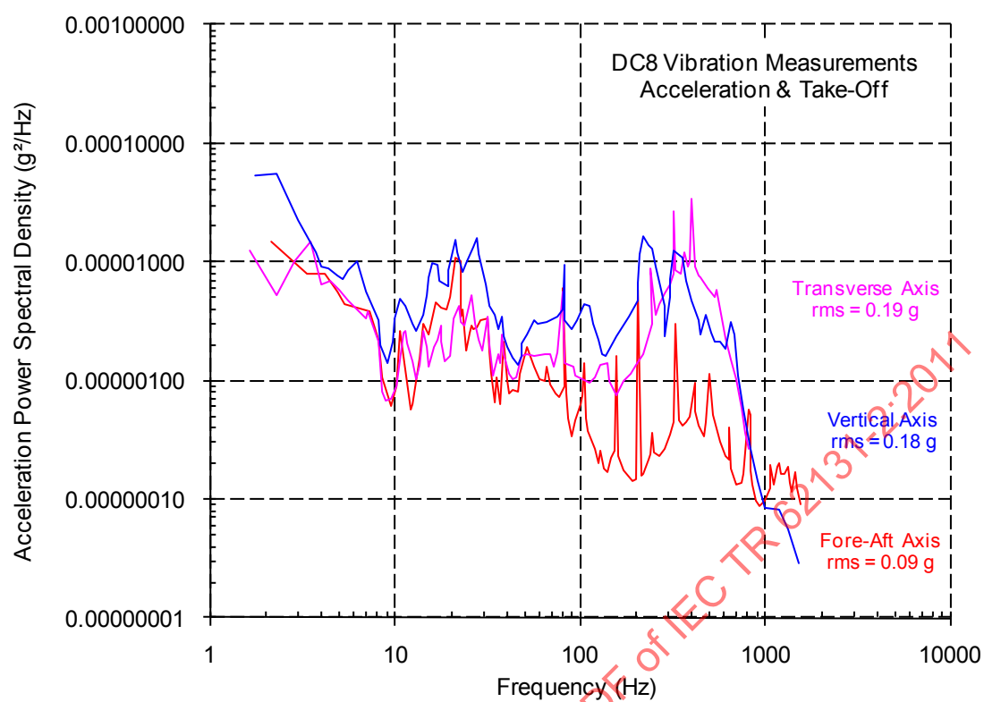
Figure 25 – DC8 vibration measurements acceleration and take-off
