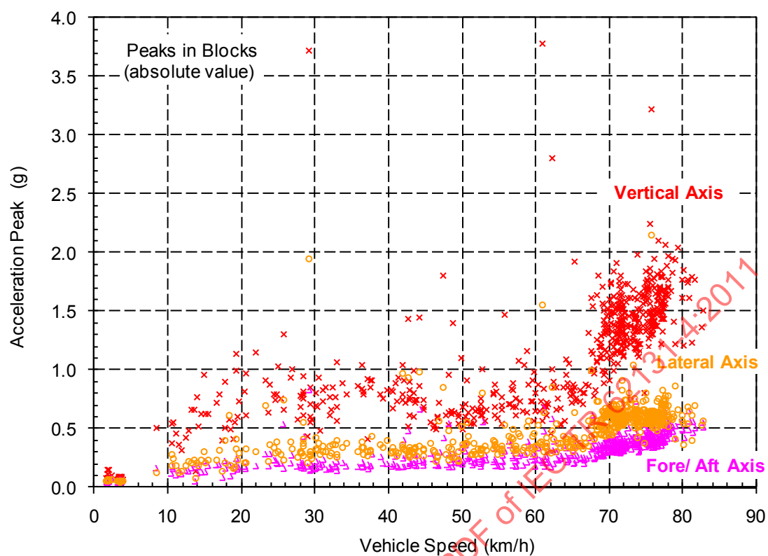
Figure 20 – Acceleration peaks against vehicle velocity for CEEES analysis
