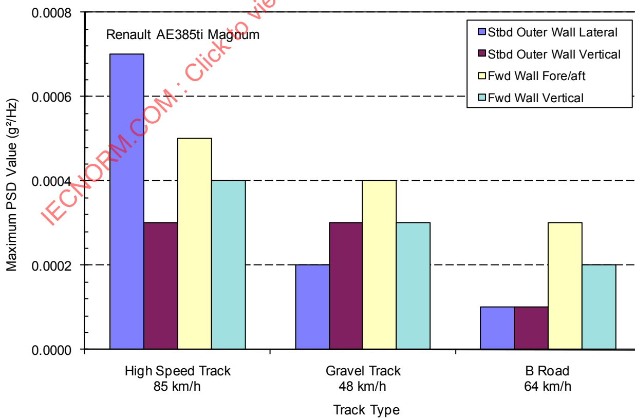
Figure 38 – Maximum PSD values from Millbrook measurements on Renault Magnum
