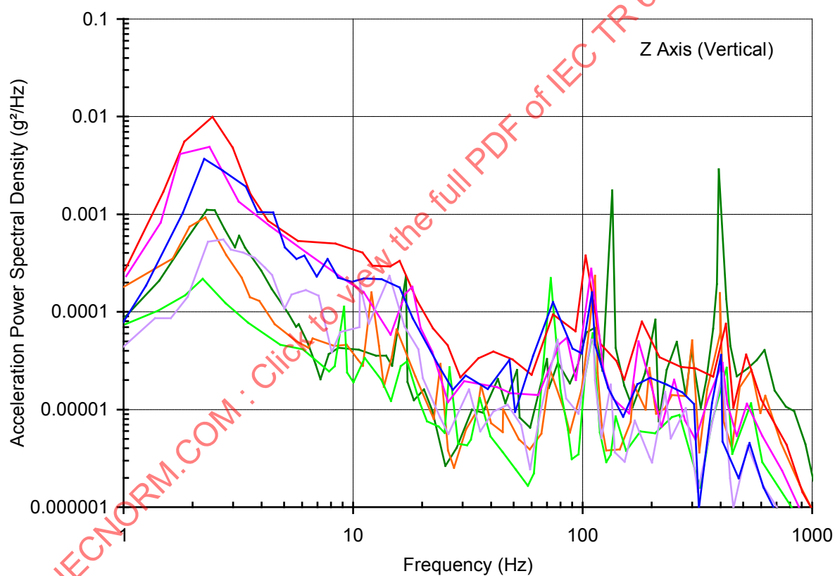
Figure 41 – Vibration PSD from GAM EG 13 measurements on Renault Traffic
