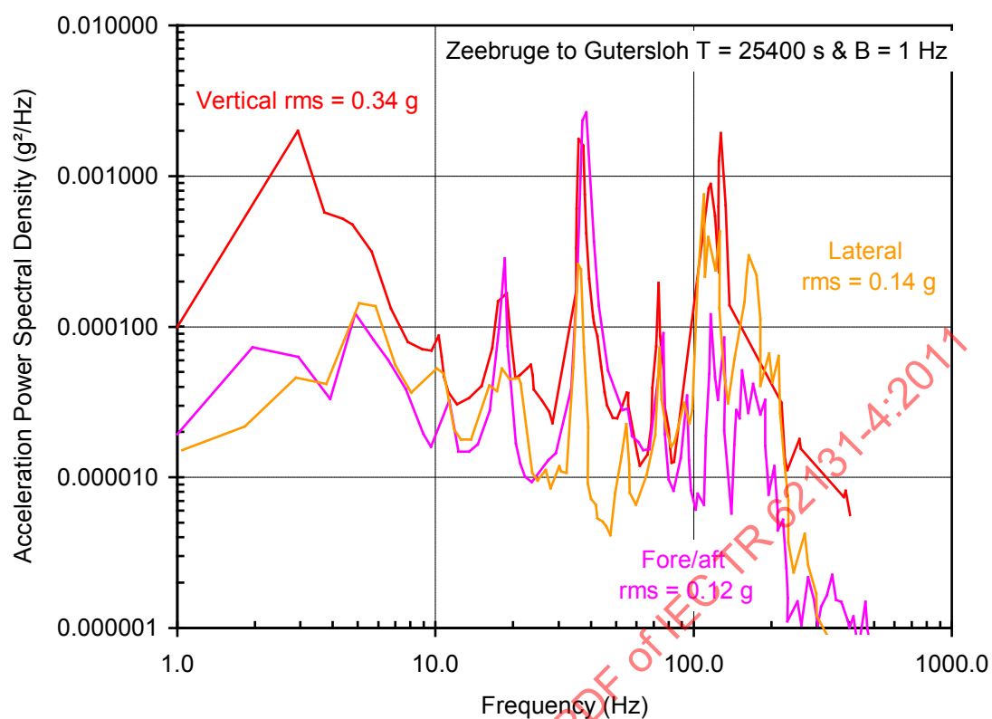
Figure 24 – Composite vibration PSD of CEEES measurements
