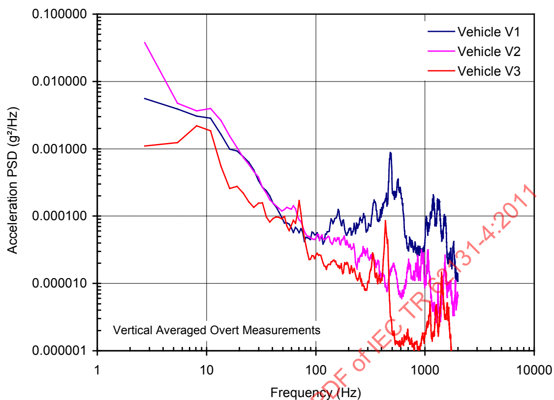
Figure 8 – Comparison of different SRETS vehicles at the load platform – Measurements made with driver's knowledge
