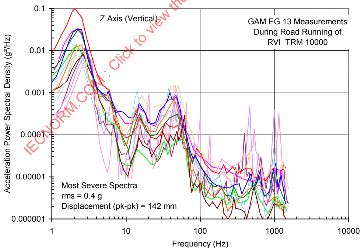
Figure 42 – Vibration PSD from GAM EG 13 measurements on RVI TRM 1000
