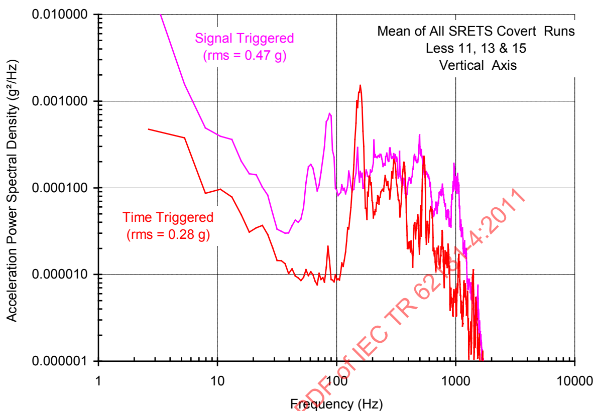
Figure 12 – Power spectral density of SRETS time and signal triggered data made without driver's knowledge
