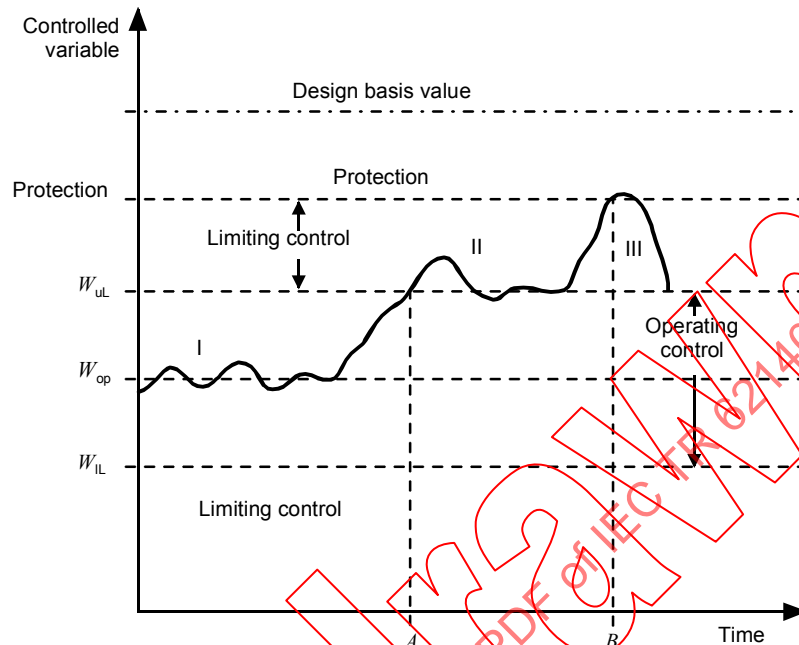
Figure 1 – Change in a controlled variable over time
