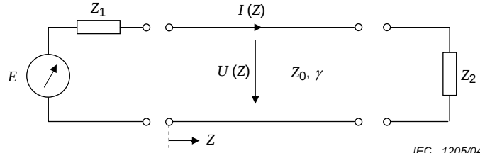
Figure C.22 – Homogenous transmission line
