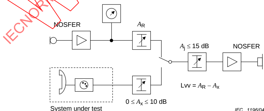
Figure C.13 – Measurement of the sending reference equivalent
