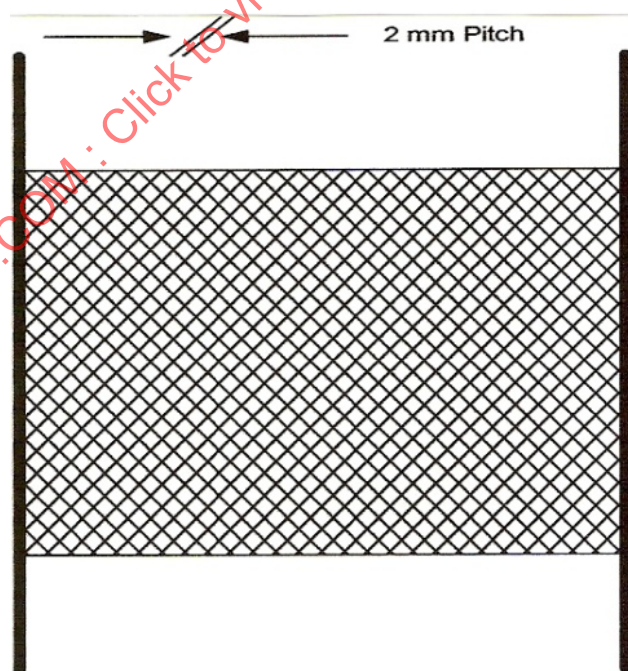
Figure 6 – Quartz drum with basketwoven fibre
