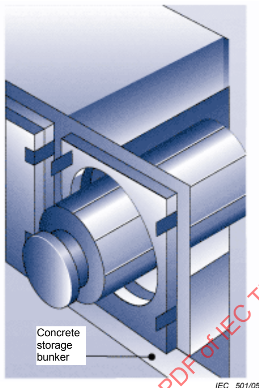
Figure 3 – Typical horizontal vault for dry storage containers
