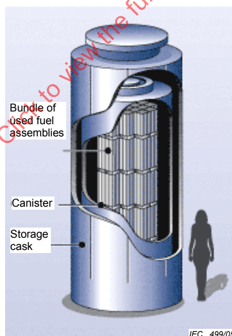
Figure 1 – Typical storage cask
