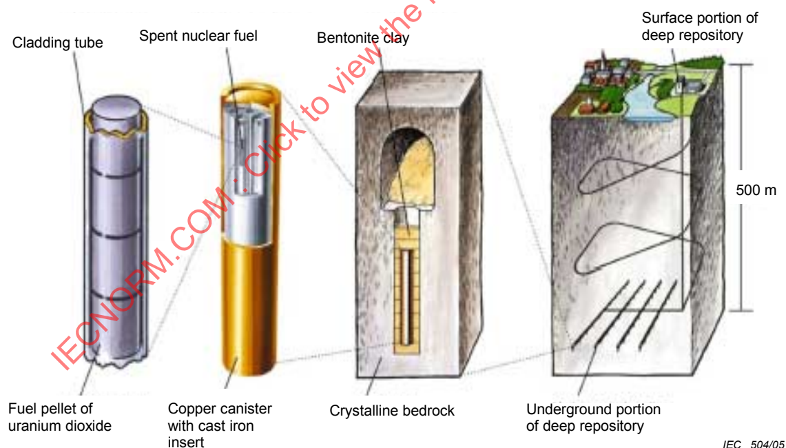
Figure 6 – Swedish system for a deep repository
