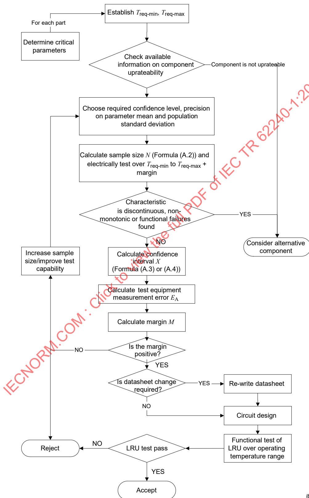
Figure A.2 – Flow diagram of parameter re-characterisation capability assurance process
