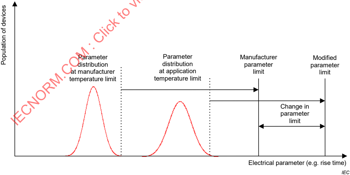
Figure A.1 – Parameter re-characterisation
