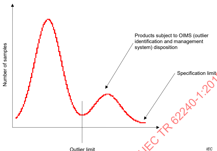
Figure A.6 – Schematic of outlier products that may can invalidate sample testing
