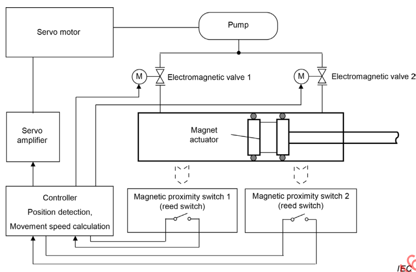
Figure A.2 – Control circuit of reed switches of magnetic proximity switches
