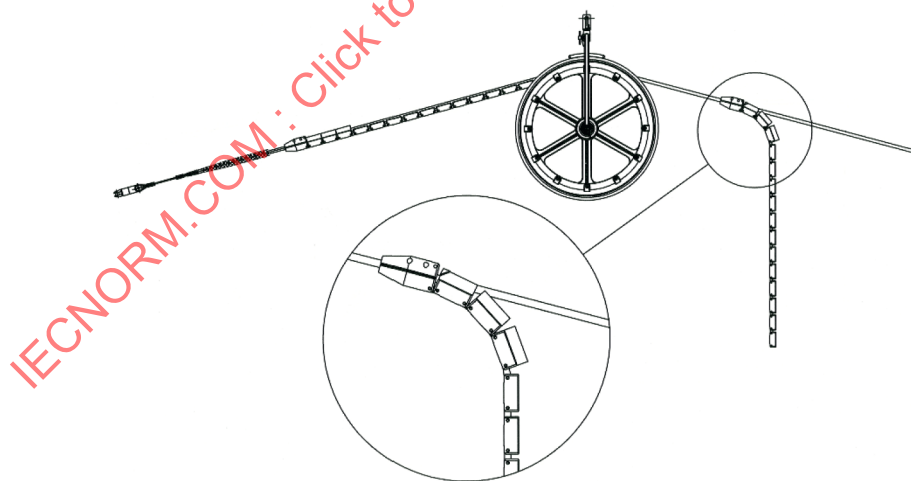
b) Clamp device to be used with articulated long shape running board
