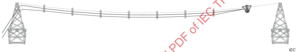
Figure 19 – Recovery of ropes and cradle blocks
