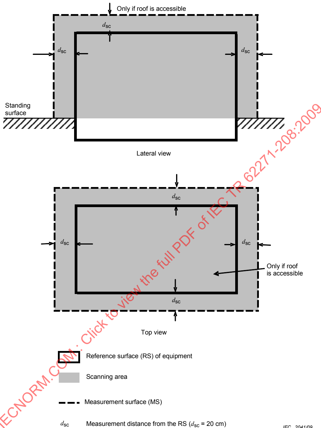
Figure 3 – Scanning areas to find the hot spots
