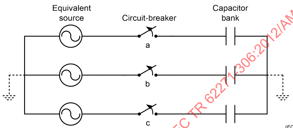
Figure 130 – Basic circuit for shunt capacitor bank switching
