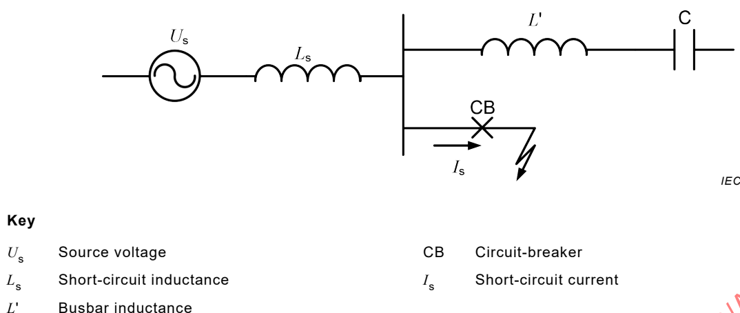
Figure 127 – Fault in the vicinity of a capacitor bank
