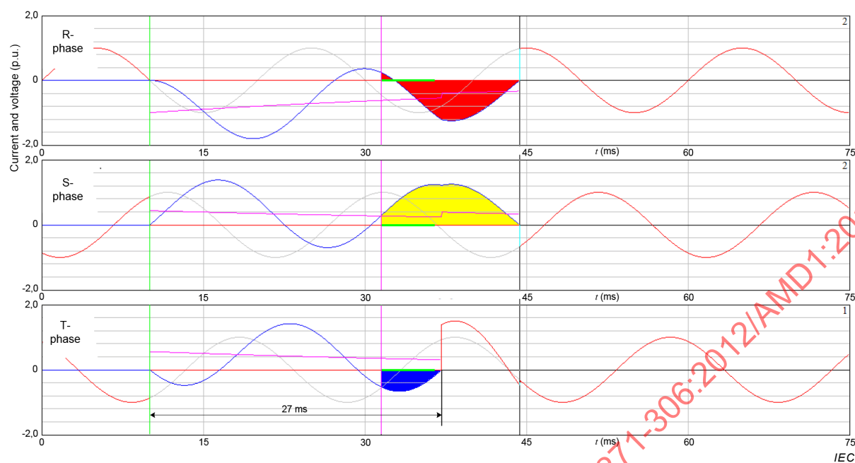
Figure 137a – Case 1 with k_{pp} = 1,5
