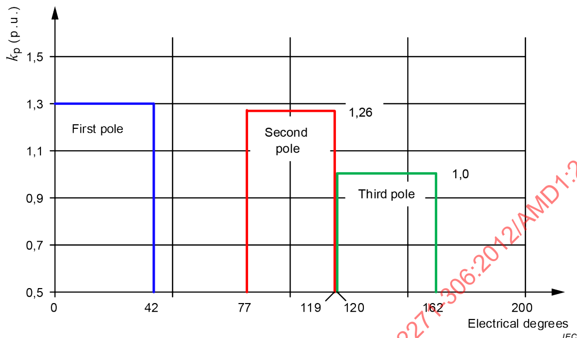
Figure 134 – Interrupting windows and k_p values for three-phase fault to earth in an effectively earthed system at 800 kV and below
