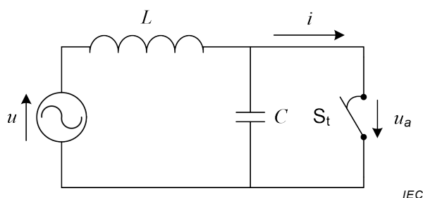
Figure 152 – Direct test circuit, simplified diagram
