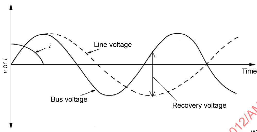
Figure 118 – Typical current and voltage relations for a compensated line
