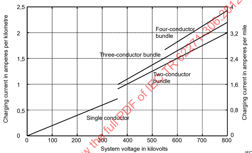
Figure 115 – RMS charging current versus system voltage for different line configurations at 60 Hz
