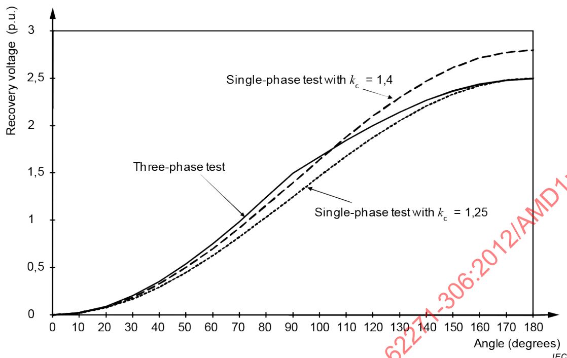
Figure 121 – Recovery voltage on first-pole-to-clear for three-phase interruption: capacitor bank with isolated neutral
