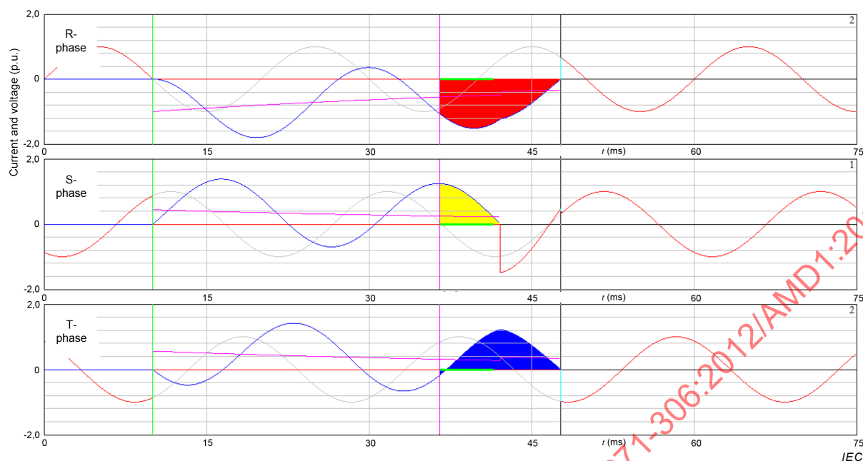
Figure 139 – Case 3 with interruption of a last pole-to-clear after a major extended loop of current with required asymmetry but not the longest arcing time
