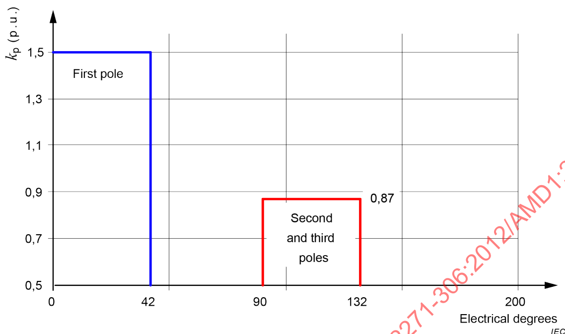
Figure 132 – Interrupting windows and k_p value for three-phase fault in a non-effectively earthed system
