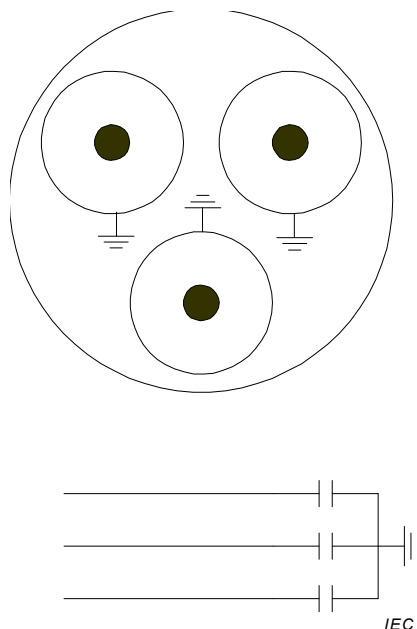
Figure 106 – Individually screened cable with equivalent circuit
