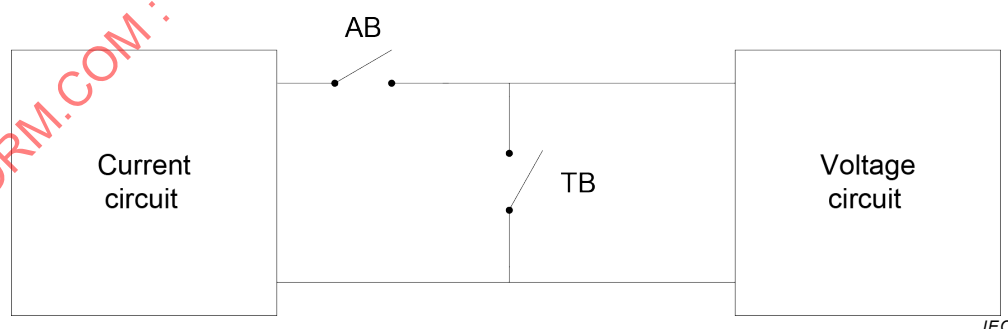
Figure 144 – Principle of synthetic testing
