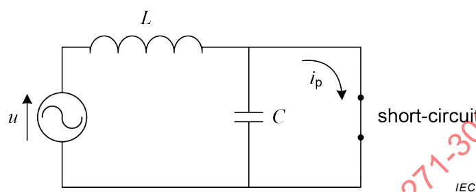
Figure 153 – Prospective short-circuit current flow
