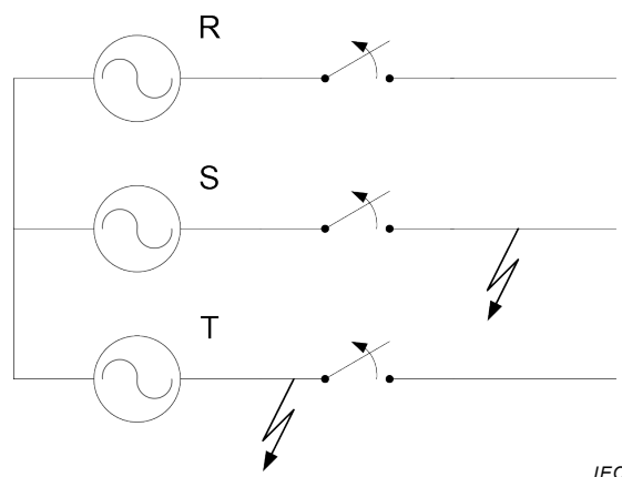
Figure 141 – Representation of a system with a double earth fault
