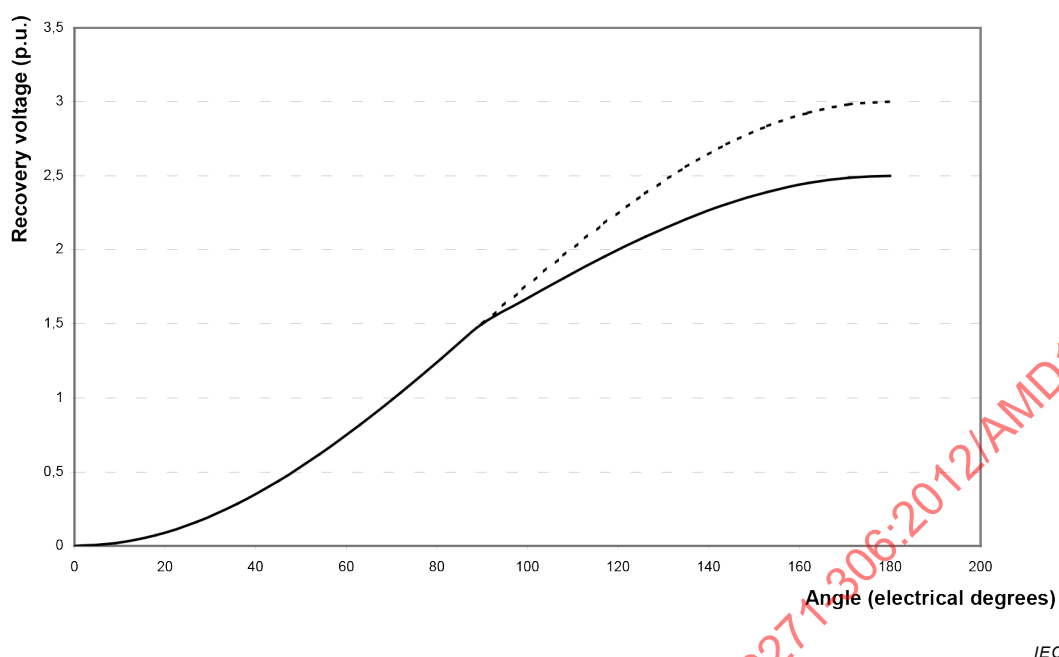
Figure 103 – Recovery voltage of the first-pole-to-clear at interruption of a three-phase non-effectively earthed capacitive load
