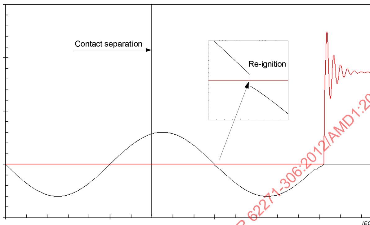
Figure 164 – Typical waveshapes obtained during a symmetrical test using the circuit in Figure 163
