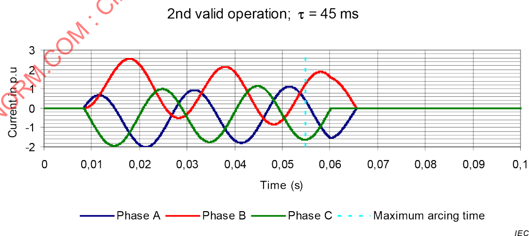
Figure A.4 – Second valid operation in case of three-phase test on a circuit-breaker exhibiting a very short minimum arcing time
