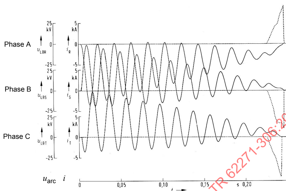
Figure B.9 – Circuit-breaker currents i and arc voltages u_{arc} under conditions of unsynchronized closing with 90^\circ differential angle
