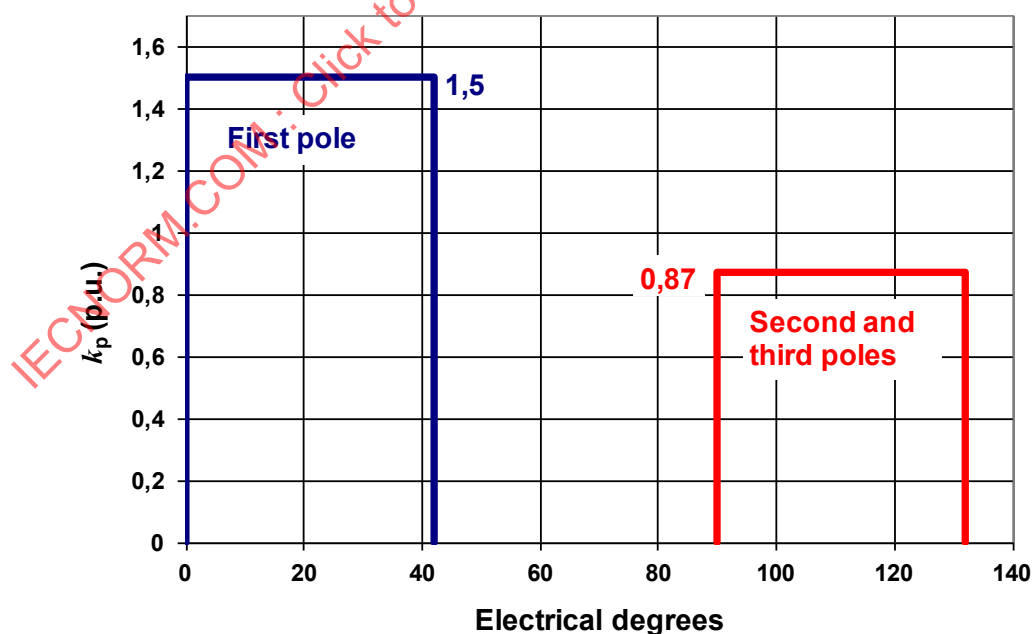
Figure 67 – Arcing windows and k_p value for three-phase fault in a non-effectively earthed system
