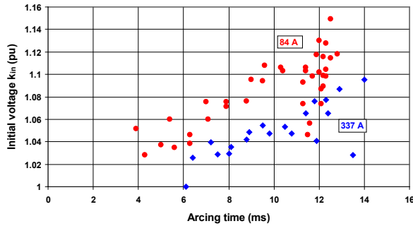
Figure 91 – Initial voltage k_{in} versus arcing time
