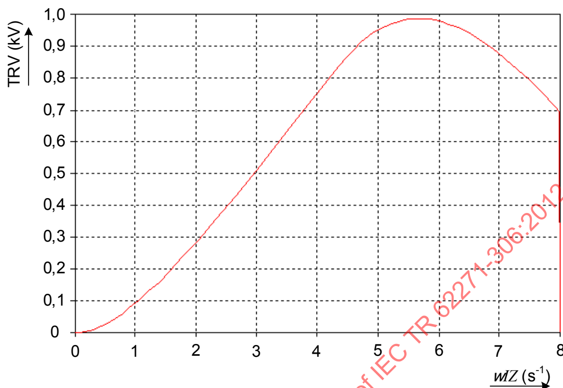
Figure 20 – TRV vs. I Z as function of t/t_{dL} when t_L/t_{dL} = 4,0
