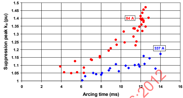
Figure 92 – Suppression peak overvoltage versus arcing time
