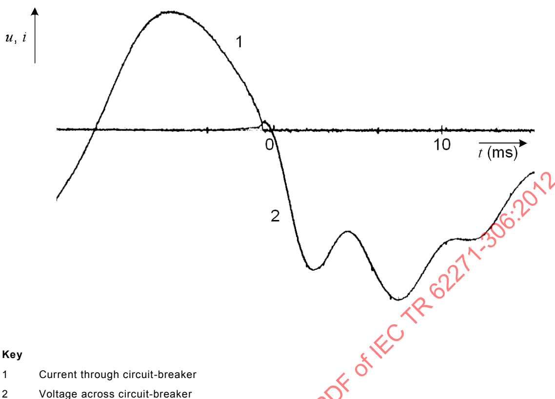
Figure 55 – Example of the recovery voltage across a filter bank circuit-breaker
