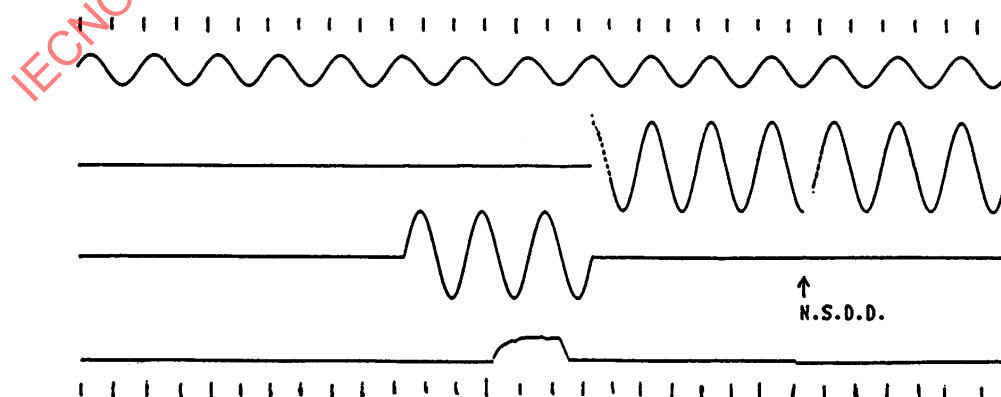
Figure 50 – NSDD in a single-phase test circuit
