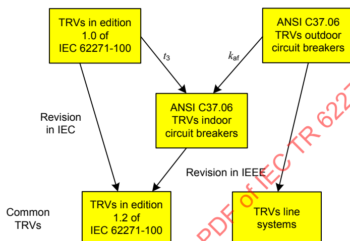
Figure 14 – Harmonization of TRVs for circuit-breakers < 100 kV
