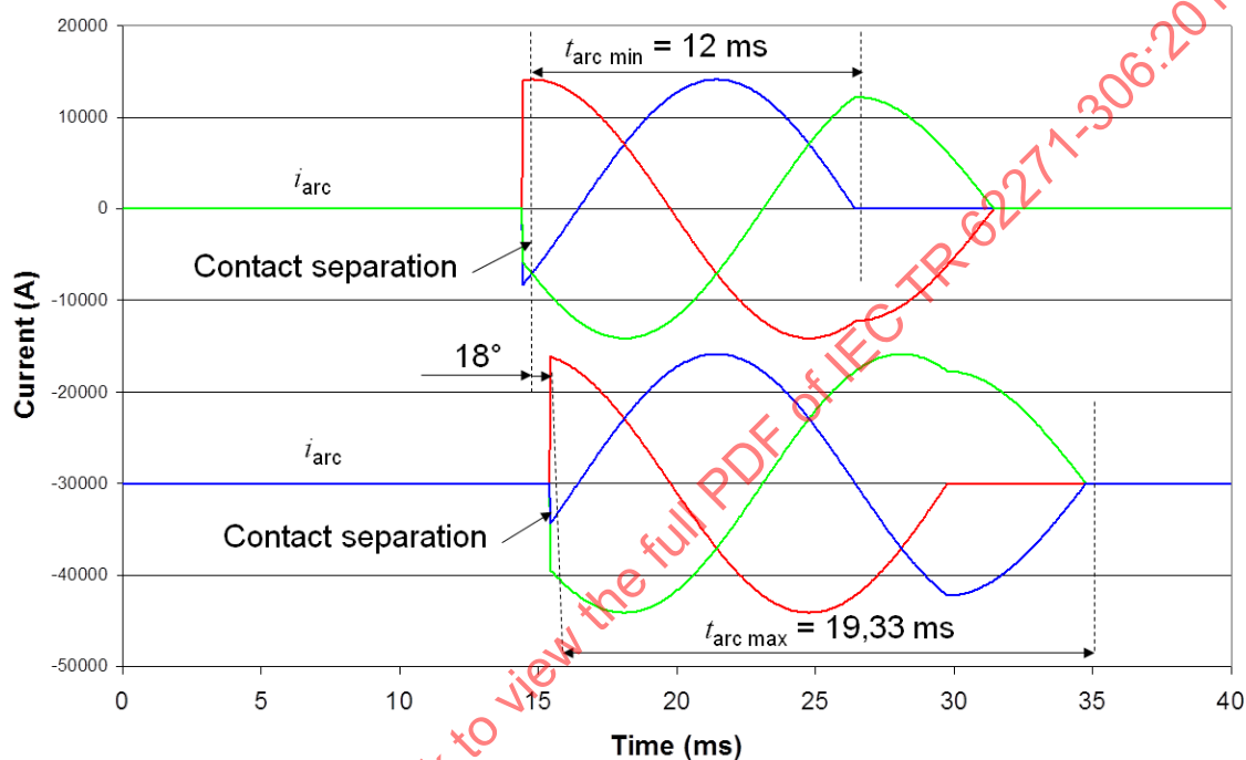
Figure 68 – Three-phase unearthened fault current interruption
