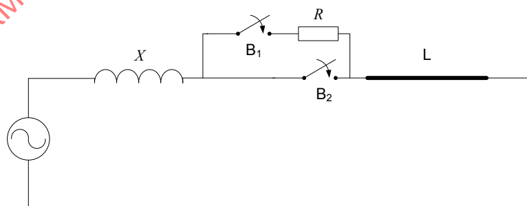
Figure 49 – Pre-insertion resistors and their function
