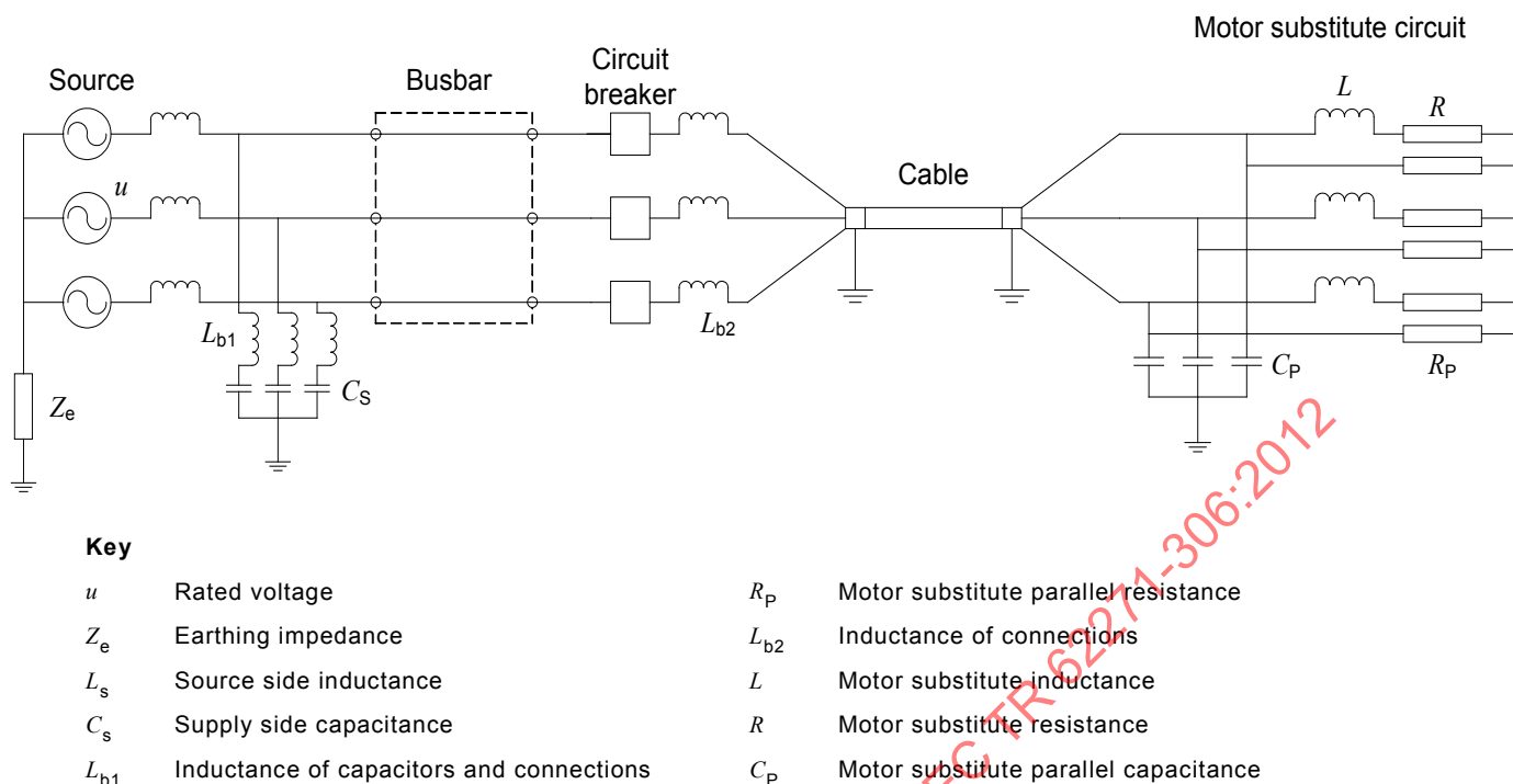
Figure 84 – Motor switching equivalent circuit
