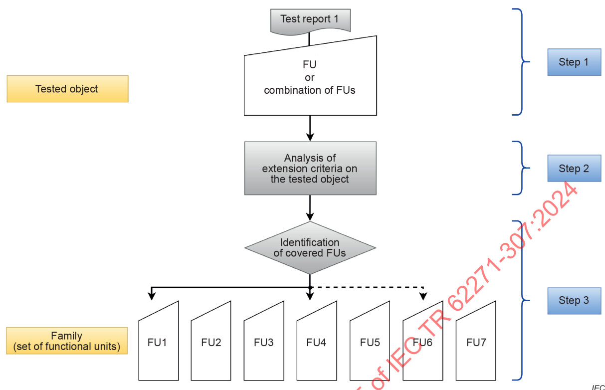
Figure 2 – Extension of validity of one test report – Situation a)
