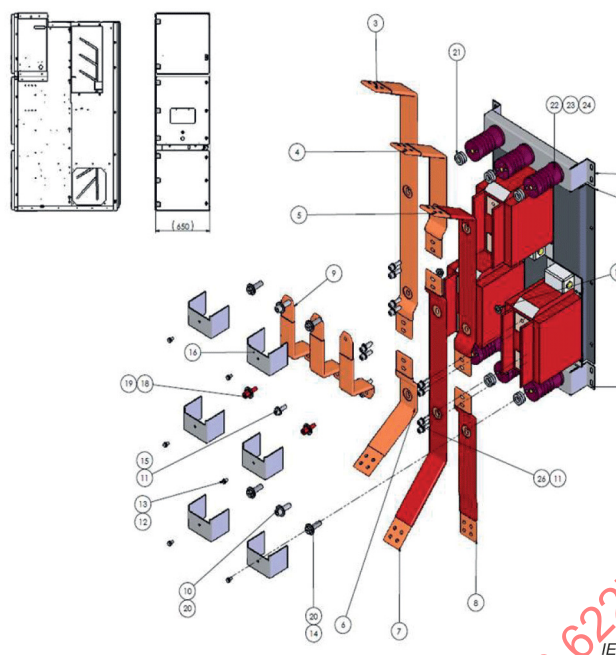
Figure B.2 – Addition of block-type current transformers into the bus riser functional unit of AIS
