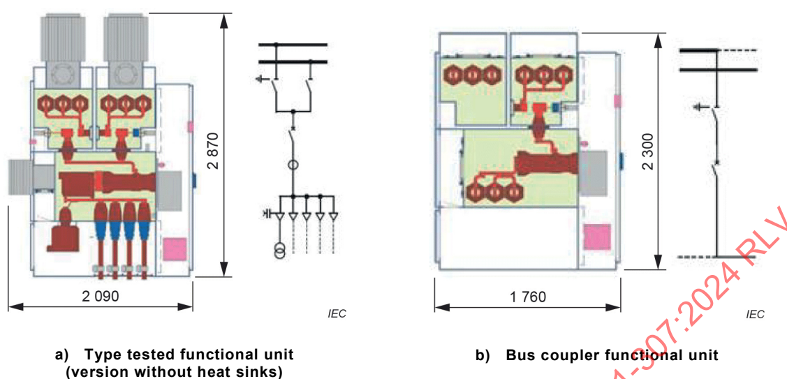
Figure B.5 – Cross-section of two different functional units of GIS
