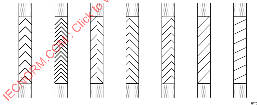
Figure A.3 – Types of ventilation opening designs
