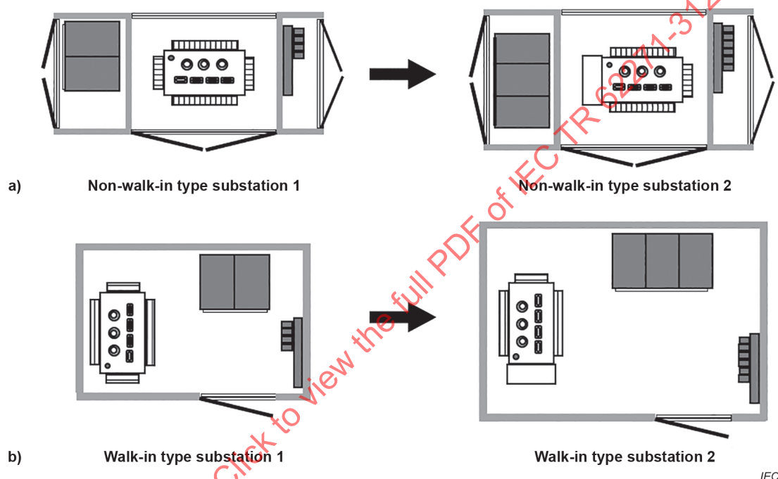
Figure A.14 – Different size of prefabricated substations with same layout
