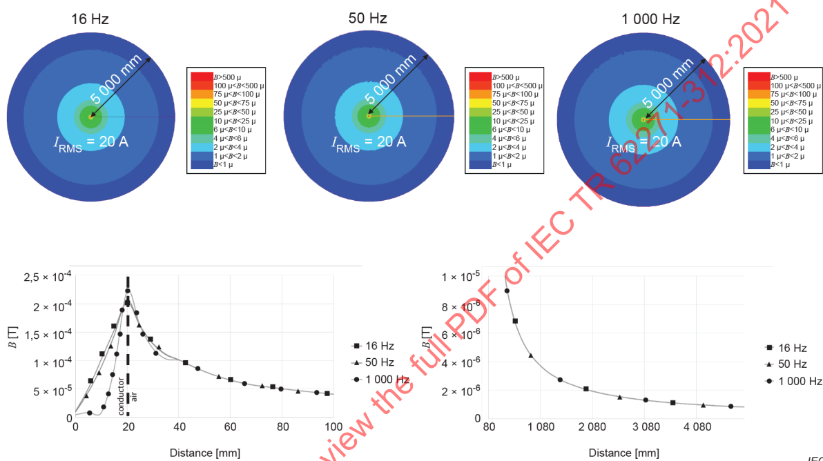
Figure A.9 – Frequency influence on magnetic field
