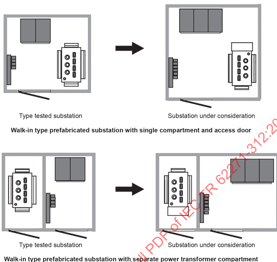
Figure A.2 – Different examples of walk-in type-tested prefabricated substation and related prefabricated substation under consideration
