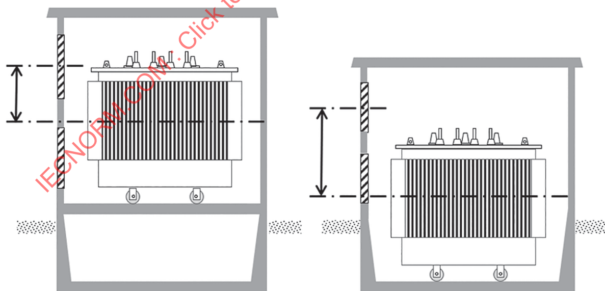
Figure A.5 – Difference in height between power transformer and air outlet ventilation openings
