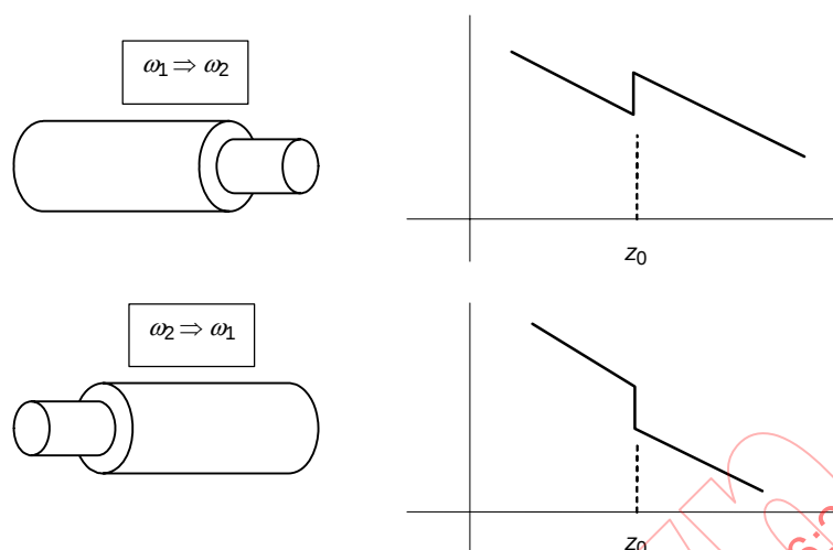
Figure 2 – OTDR traces for fibres with different MFD
