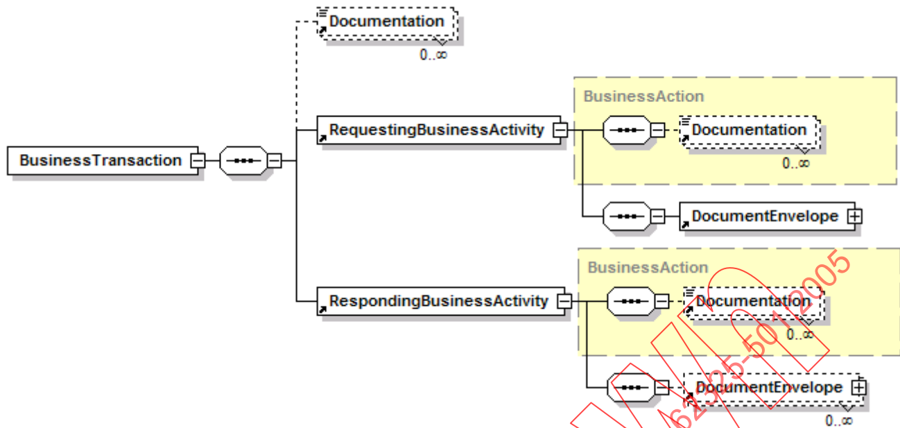
Figure 2 – Business transaction
