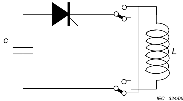
Figure 4 – Unidirectional pulses (1/2 sine wave) electrical configuration
