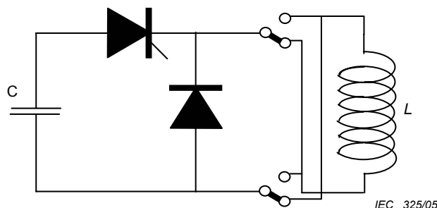
Figure 5 – Unidirectional pulses (decaying) electrical configuration
