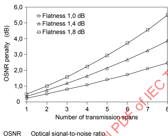
Figure 3 – OSNR penalty caused by optical gain non-uniformity
