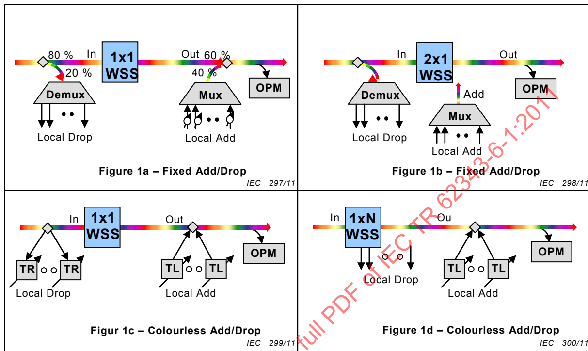
Figure 1 – ROADM architecture
