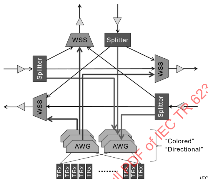
Figure 13 – Coloured and directional ROADM architecture including WSS, splitters, AWGs and transceivers (TRx)
