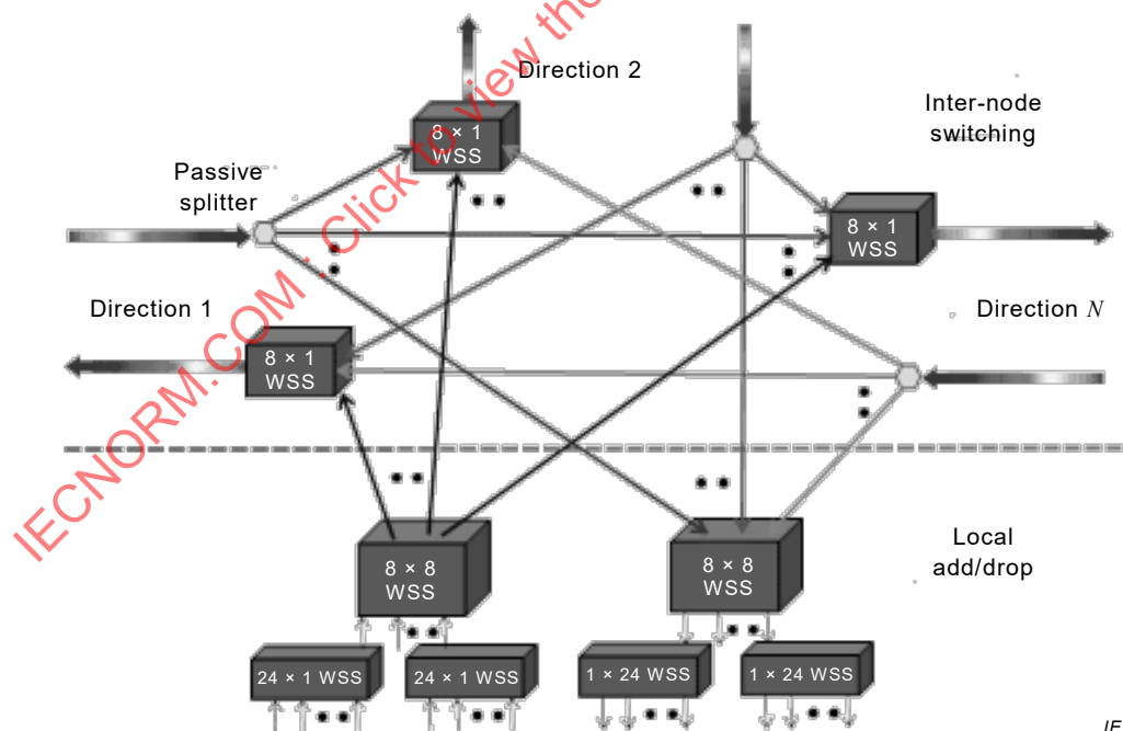
Figure 12 – 8 \times 8 WSS and large port count 1 \times 24 WSS based colourless, directionless and contentionless ROADM architecture
