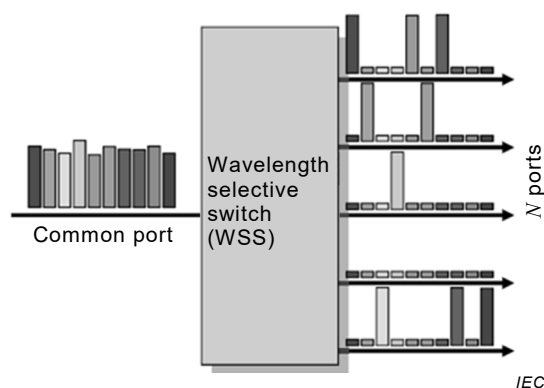
a) 1 \times N wavelength selective switch functionality
