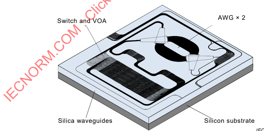
Figure A.1 – Example of PLC devices for ROADM systems
