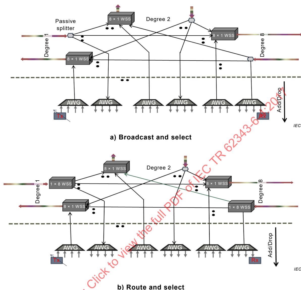
Figure 11 – ROADMs route and select architectures
