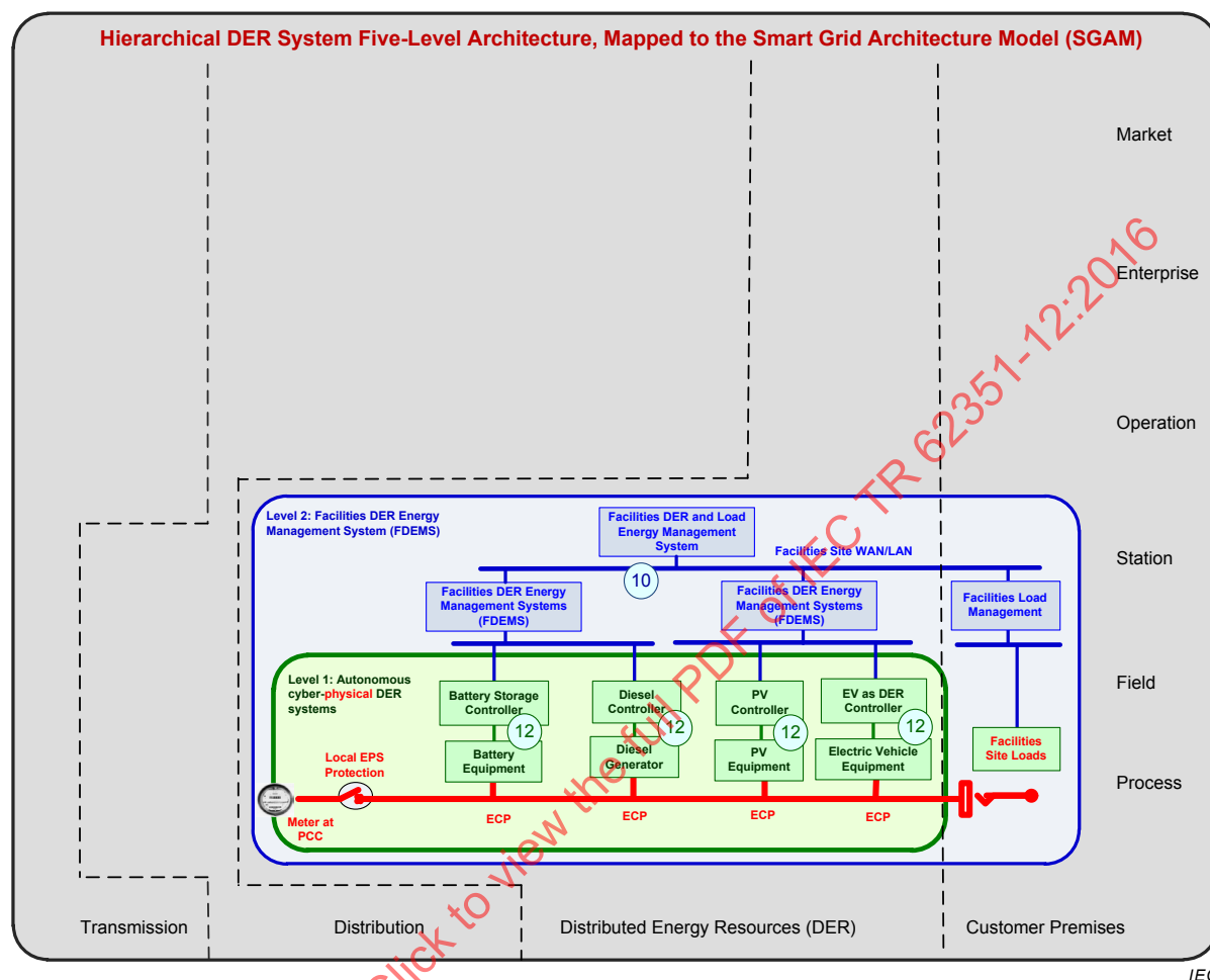
Figure 8 – Level 2 FDEMS architecture
