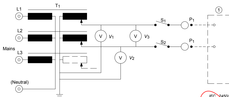
Figure D.4 – Measuring supply circuit for single-phase ME EQUIPMENT specified for connection to a polyphase SUPPLY MAINS (IEC 60601-1:2005, Figure F.4)
