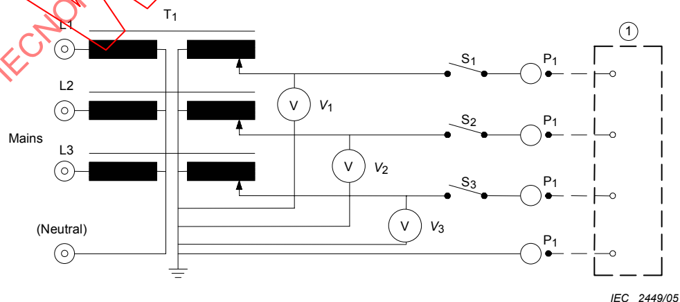
Figure D.2 – Measuring supply circuit with SUPPLY MAINS approximately symmetrical to earth potential (IEC 60601-1:2005, Figure F.2)
