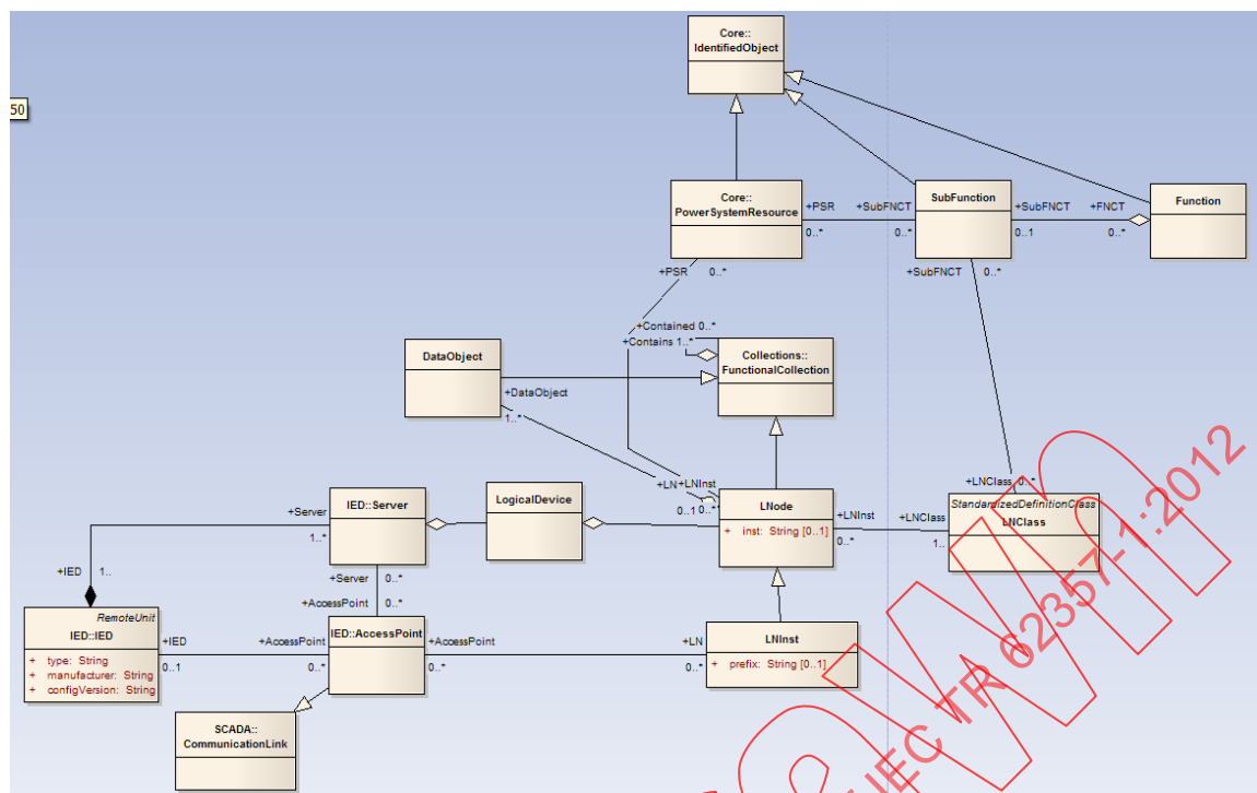
Figure 26 – Proposed linkage of IEC 61850 classes to CIM PSR classes in UML
