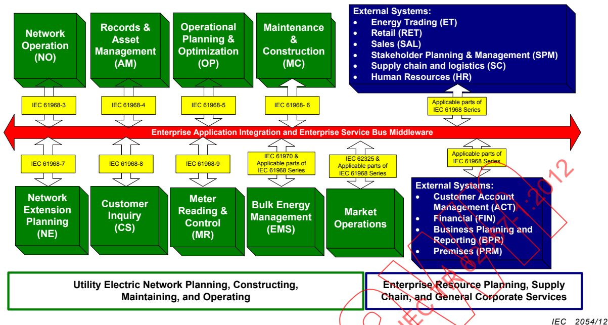
Figure 6 – IEC 61968 Interface Reference Model (IRM)
