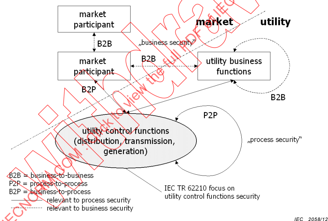
Figure 10 – Framework for deregulated energy market communications
