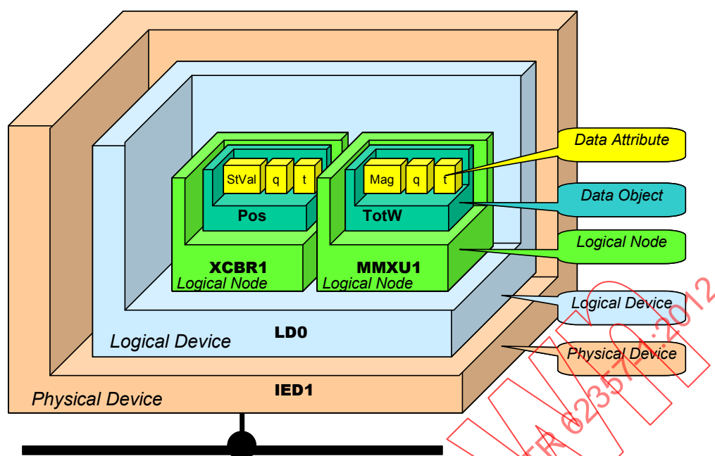
Figure 21 – IEC 61850 data modelling
