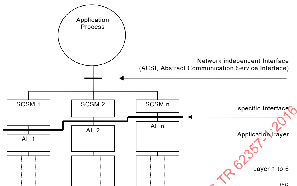
Figure 40 – Mapping of an ACSI service
