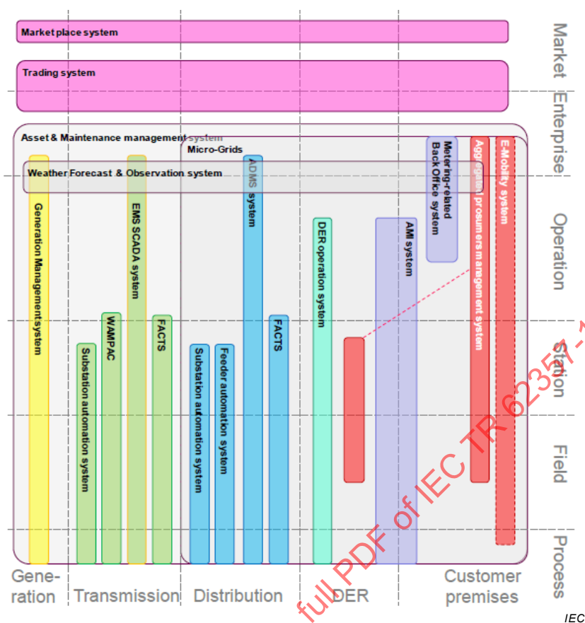
Figure 15 – SGCG/M490 Smart Grids systems on SGAM Plane
