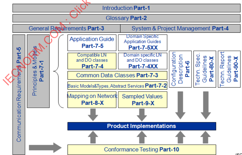
Figure D.1 – IEC 61850 standard series
