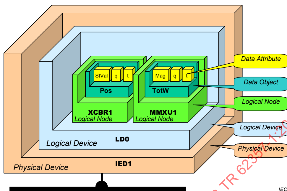
Figure 16 – IEC 61850 Data Modelling
