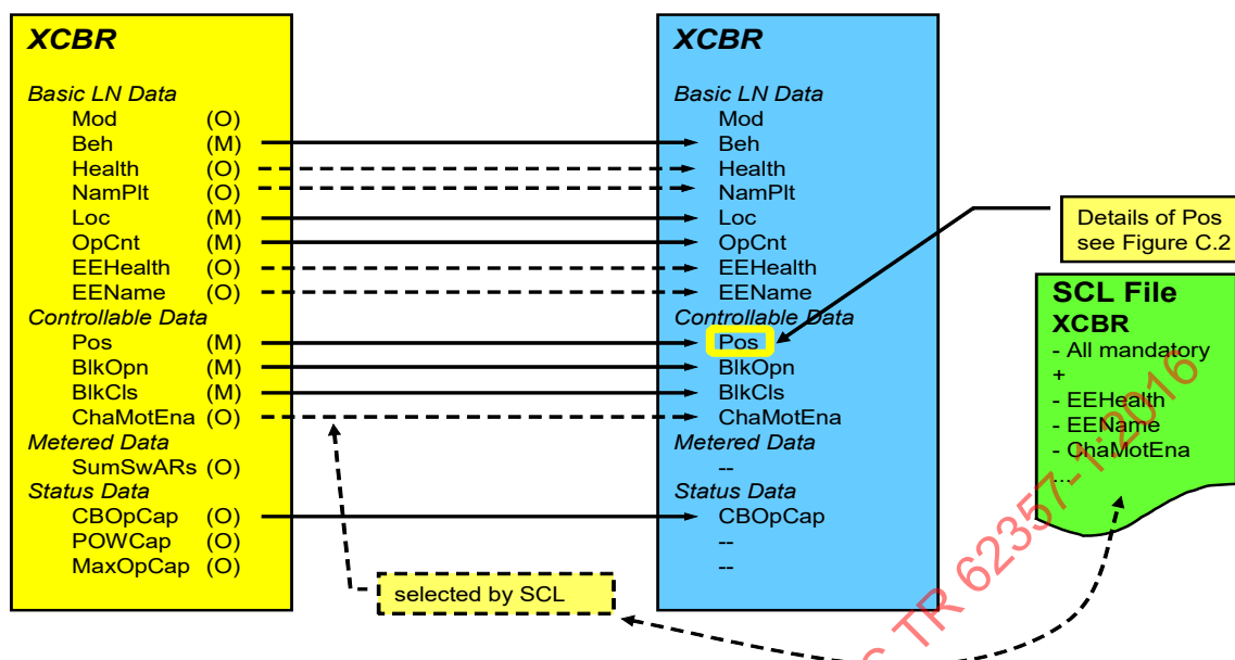
Figure 37 – SCL for LNs
