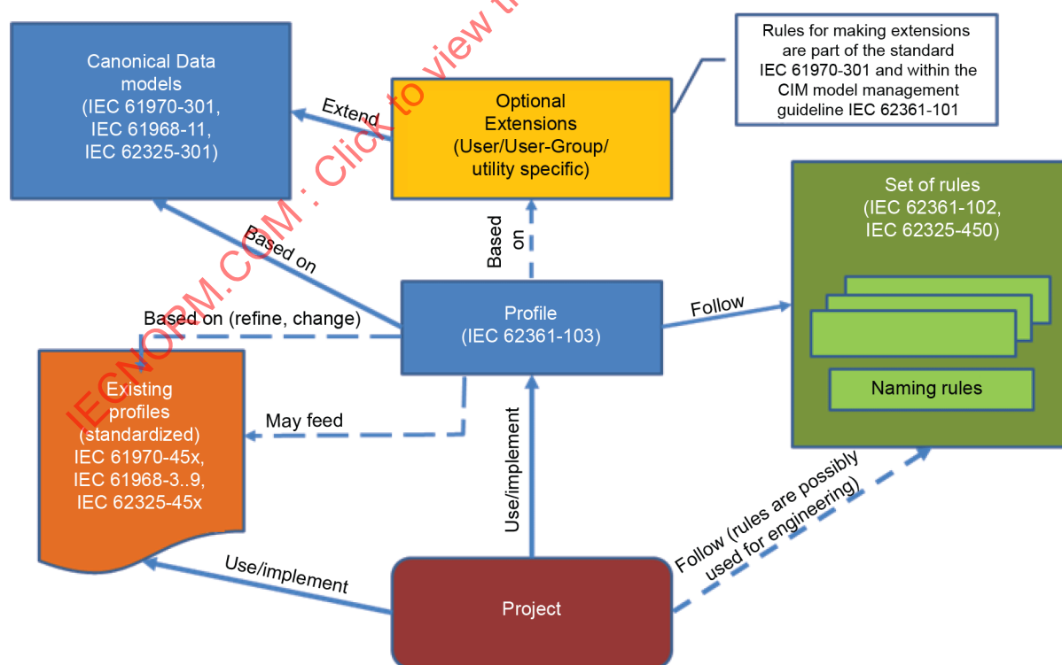
Figure 5 – Framework for profiling CIM
