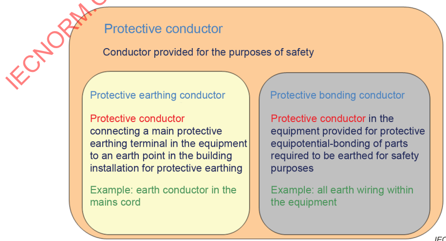
Figure 23 – Overview of protective conductors
