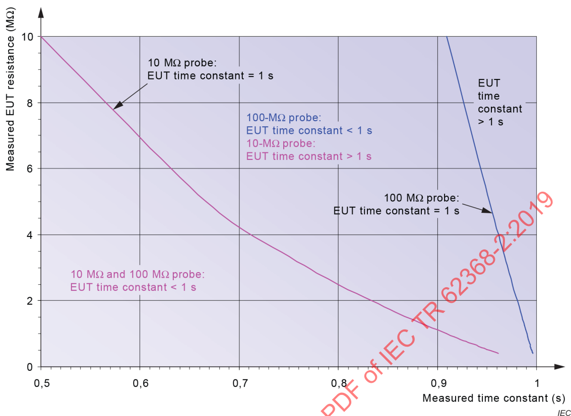
Figure B.6 – Worst-case measured time constant values for 100 M \Omega and 10 M \Omega probes
